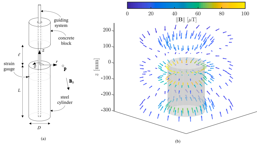
Fig. 1. (a) Schematic of the set-up of the thin-walled cylinder, including the background field B_0 . (b) Measured magnetic stray field in the vicinity of the top of the cylinder after five impacts from \ell = 1000 mm (test 2e).
