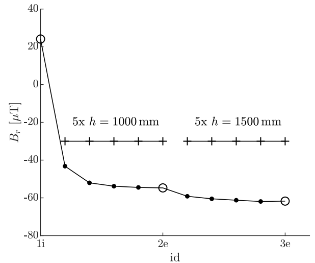
Fig. 3. Measured evolution of the radial component of the remanent stray field at z = -200 mm, r = 223.2 mm and \theta = 120^\circ for the first three tests showing the intermediate values after each impact.
