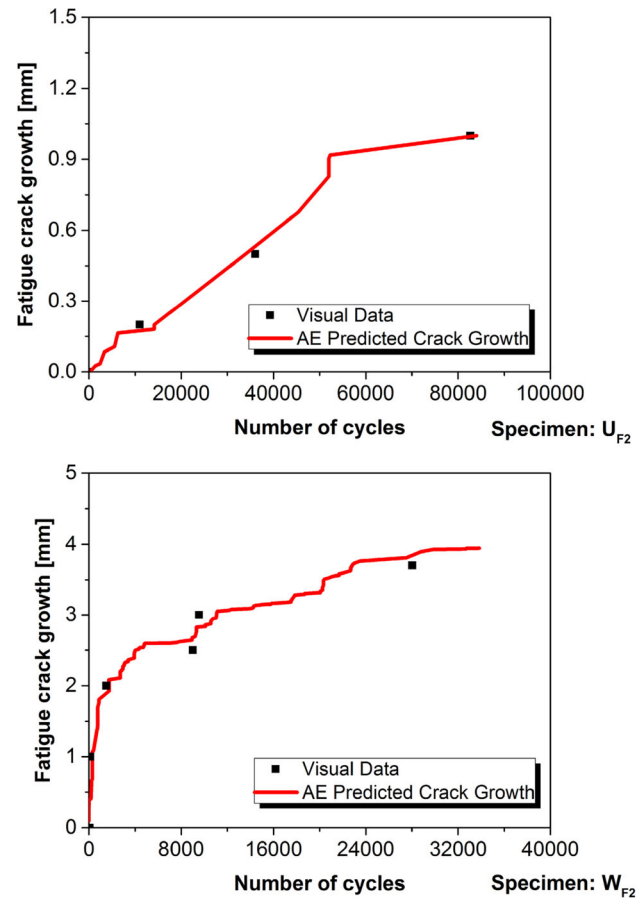
Fig. 18 Predicted and visually detected delamination fatigue crack growth for the U_{F2} and W_{F2} specimens
