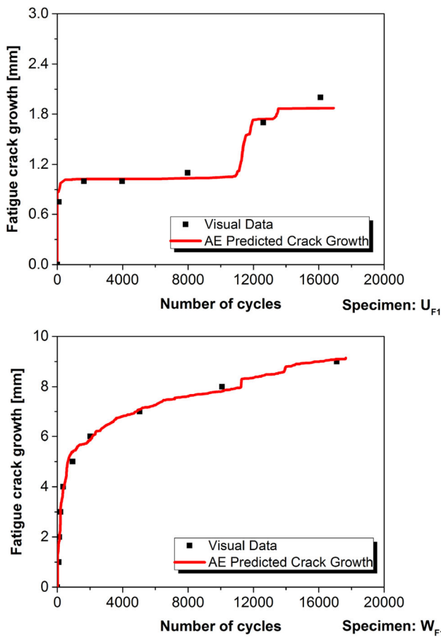
Fig. 17 Predicted and visually detected delamination fatigue crack growth for the U_{F1} and W_{F1} specimens
