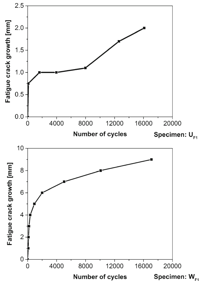
Fig. 14 The fatigue crack growth for the U_{F1} and W_{F1} specimens
