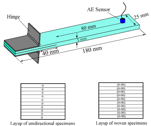
Fig. 1 The specimens geometry and dimensions
