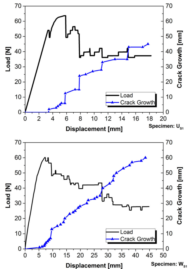
Fig. 3 Load-displacement and crack growth-displacement diagrams for the U_{S1} and W_{S1} specimens
