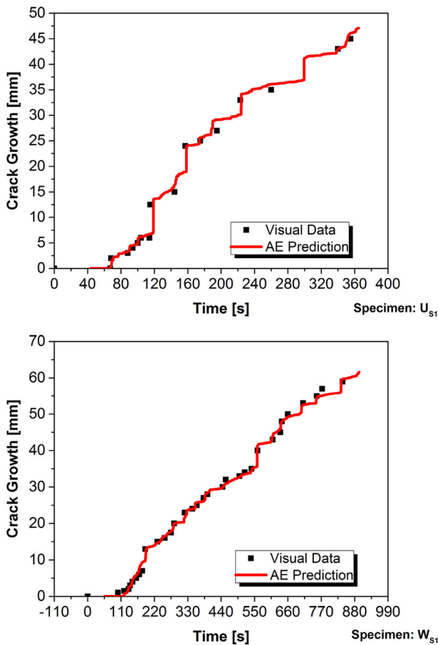
Fig. 12 Prediction of crack growth using the AE method for the U_{S1} and W_{S1} specimens
