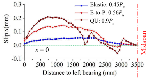
Fig. 24. Longitudinal distribution of the slip at different stages
