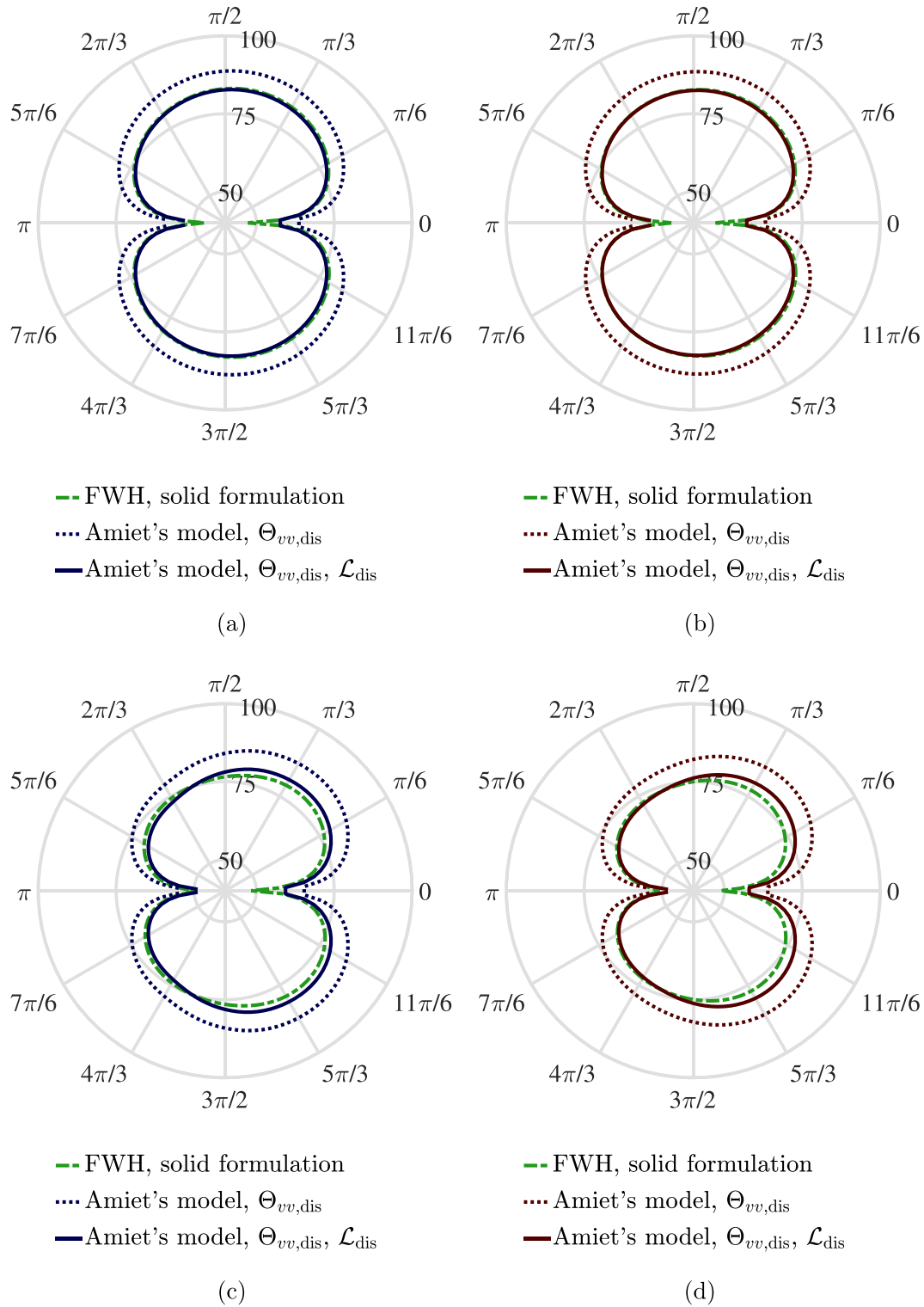
FIG. 23. Far-field noise directivity patterns in the low-frequency range St_l = [0.15, 0.35] for (a) NACA 0012 and (b) NACA 0012-103 and in the high-frequency range St_l = [0.35, 1.5] for (c) NACA 0012 and (d) NACA 0012-103. Amiet's model implementations using the distorted spectrum as input with and without the corrected transfer function are compared with the FWH results.
