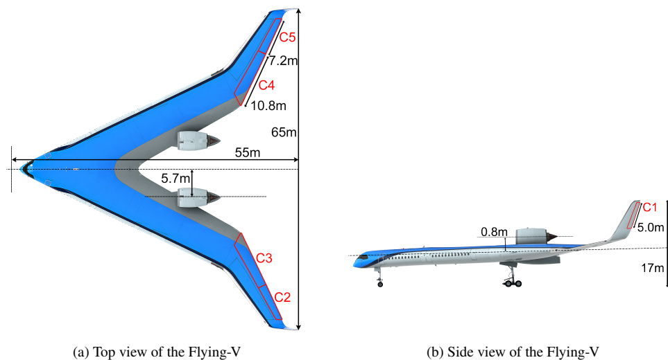
Fig. 1 Flying-V impressions and dimensions*.
