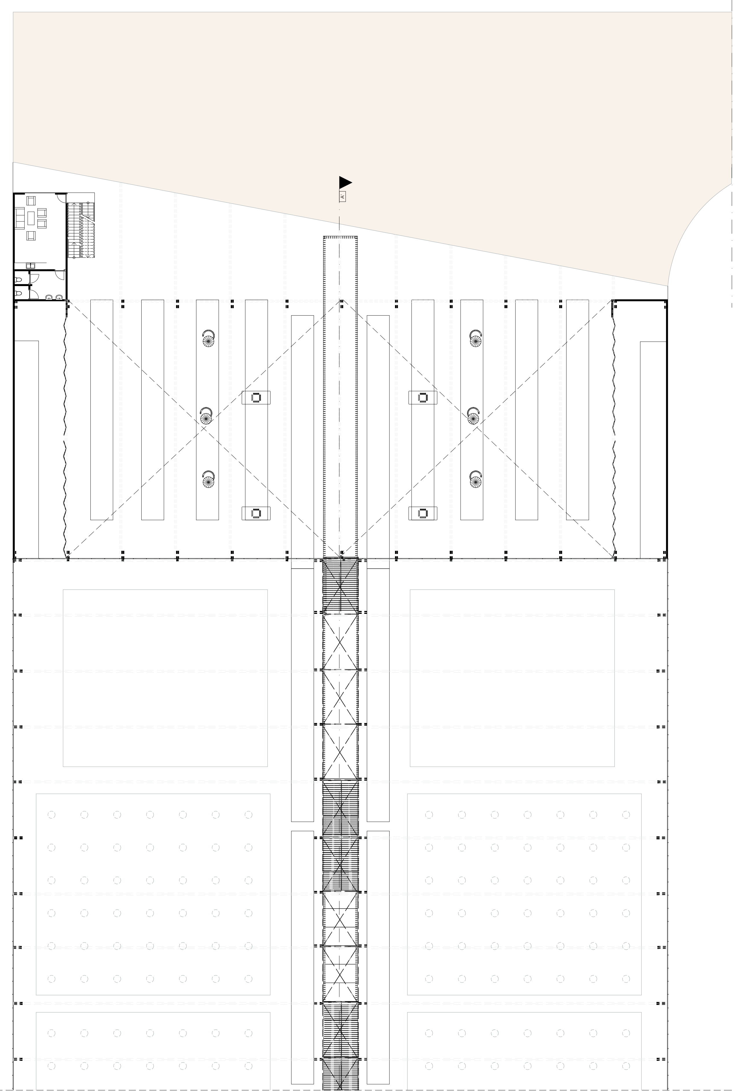
Factory building floorplan level 01
