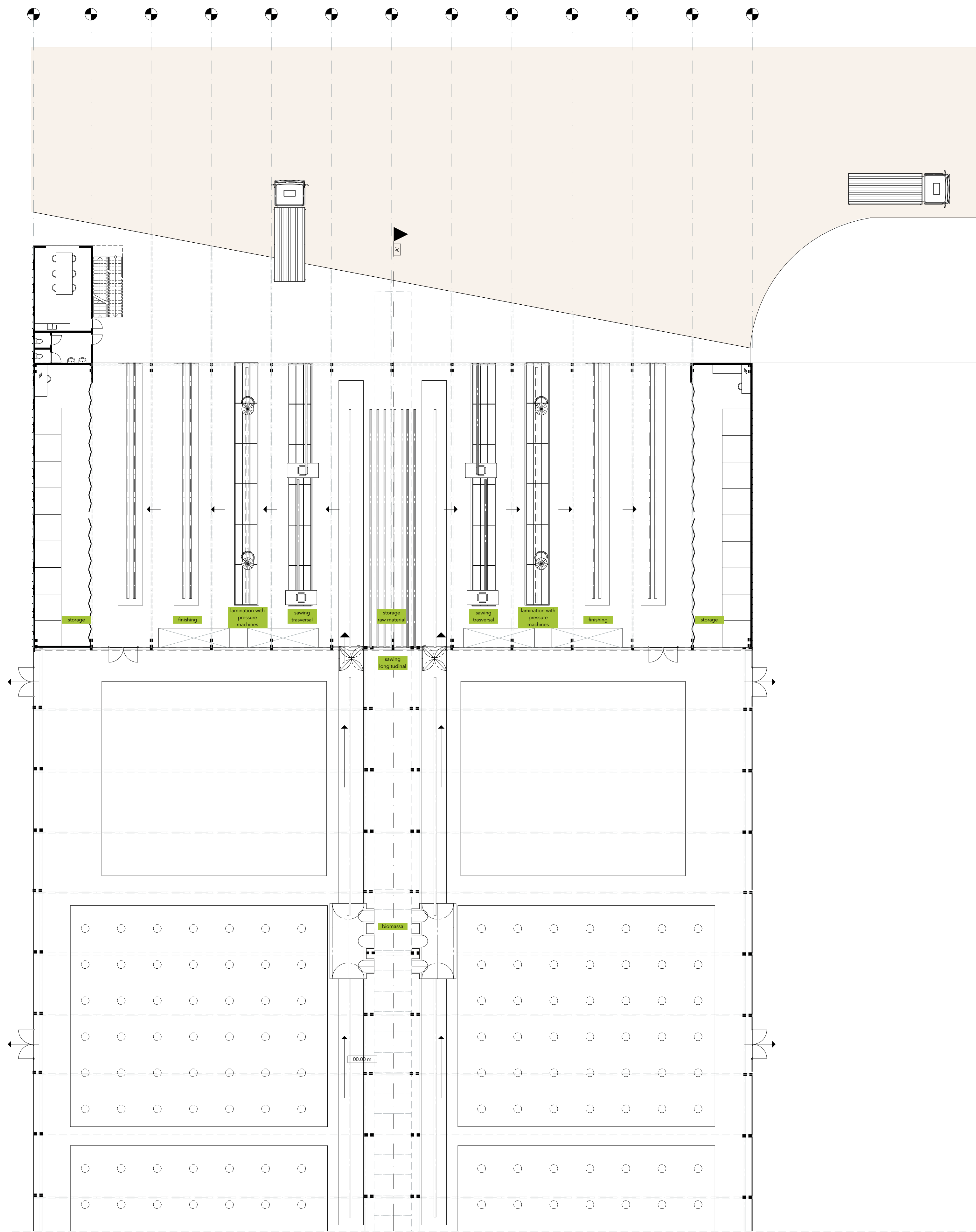
Factory building floorplan level 00
