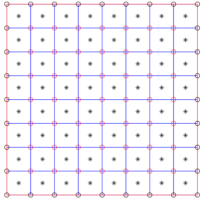
FIGURE 2 The grid for the 2D Navier–Stokes discretization
