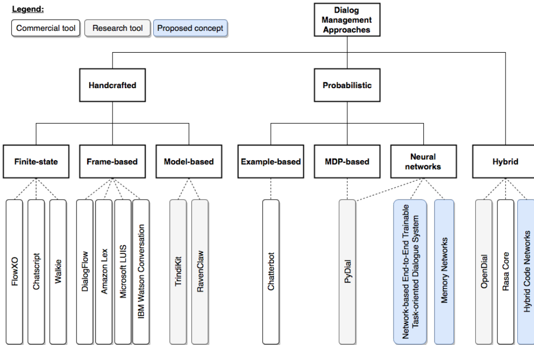
Figure 2 - Taxonomy of dialog management approaches. On the top-level three different approaches can be identified, namely handcrafted systems, statistical systems and hybrid systems. Below the subcategories, available commercial tools (white boxes), research tools (grey boxes) and research prototypes (blue boxes) are present.
