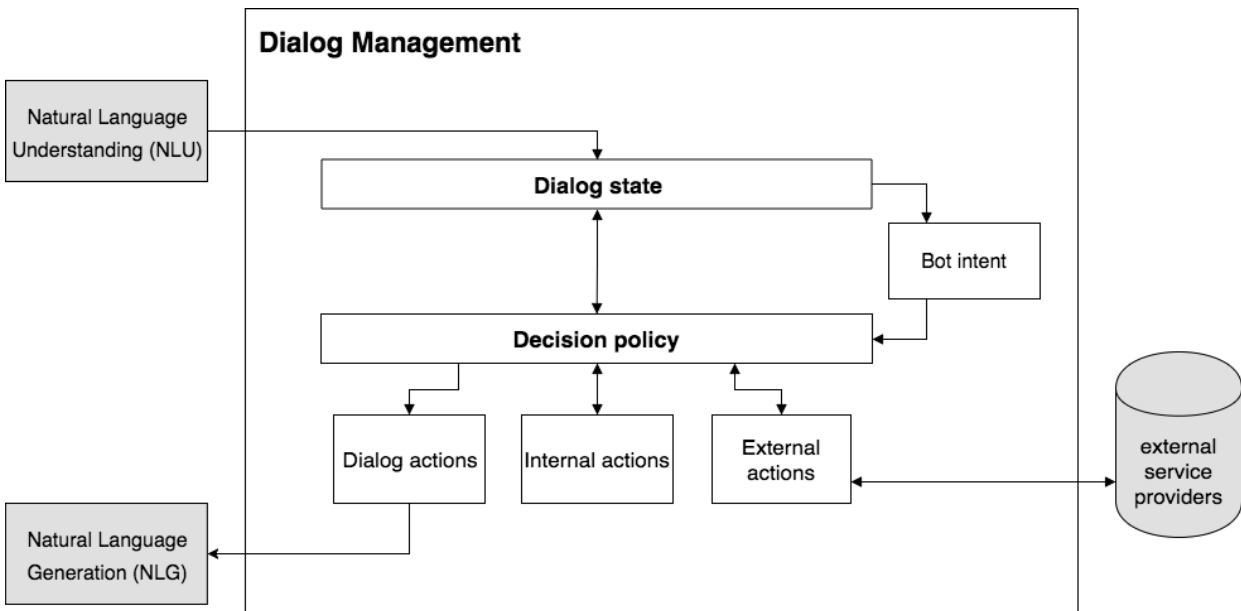
Figure 1 - Dialog management system architecture and information flow
