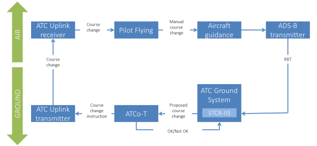
Figure 2. Information flow in the tactical layer of iA3G ConOps; STCR-IIS is part of the ATC ground system.
