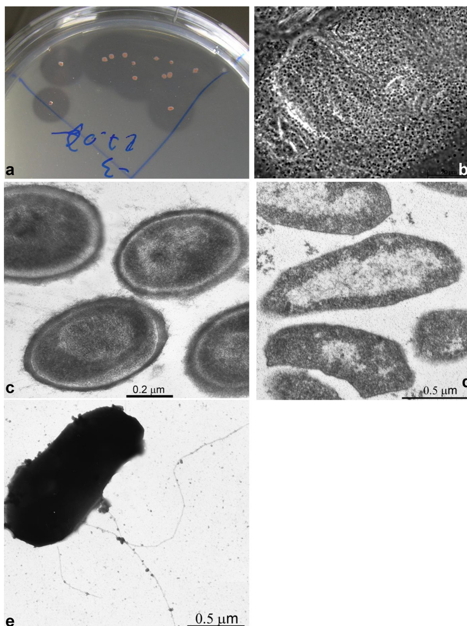
Fig. 1. Cell morphology of strain AArce15 growing on amorphous cellulose at pH 9.5, 4 M total Na + and 37 °C. (a) colonies; (b) phase contrast and (c) electron microscopy of thin sections of cells during absorption phase on cellulose; (d) electron microscopy of thin sections and (e) and whole free suspended cells from the second growth phase on cellulose.
