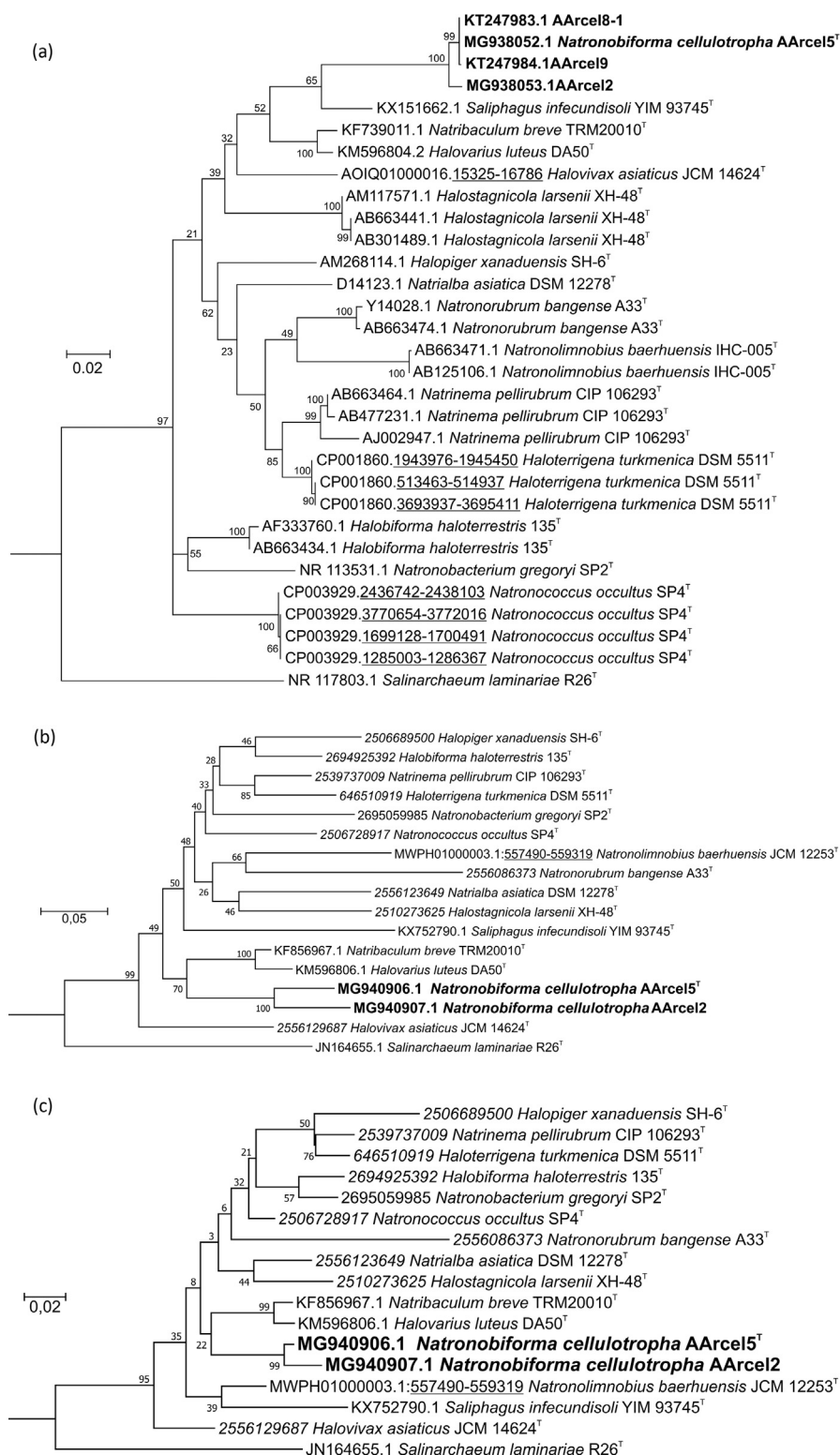
Fig. 3. Phylogeny of the AArceI strains. (a) Maximum Likelihood 16S rRNA gene sequence-based phylogenetic tree showing position of the AArceI strains (in bold) within the family Natribacteriaceae. Branch lengths (see scale) correspond to the number of substitutions per site with corrections, associated with the model (GTR, G + I, 4 categories). All positions with less than 95% site coverage were eliminated. Totally 1359 positions were used in the alignment of 32 sequences (except for the partial AArceI4 and AArceI6 sequences, 100% identical to AArceI5 T ). Numbers at nodes indicate bootstrap values of 1000 repetitions. Halomarina orientis strain JCM 16495 (AB663390.1) was used as an outgroup. (b) Maximum Likelihood rpoB' gene sequence-based tree showing position of the AArceI2 and AArceI5 strains (in bold) within family Natribacteriaceae. Totally 1827 positions were used in the alignment of 18 sequences. Halomarina orientis JCM 16495 (KJ870934.1) was used as an outgroup. (c): Maximum Likelihood RpoB' protein sequence-based tree showing position AArceI2 and AArceI5 strains (in bold) within the family Natribacteriaceae. Totally 608 positions were used in the alignment of 18 sequences. Halomarina orientis JCM 16495 (KJ870934.1) was used as an outgroup. Sequences with accession numbers in italic were obtained from IMG, in roman – from the Genbank.
