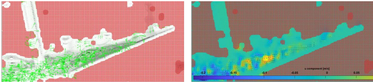
Figure 2. Left: inverted and masked image for 1:2 sloping dike. Right: reconstructed velocity field using PIVLab from Matlab.
