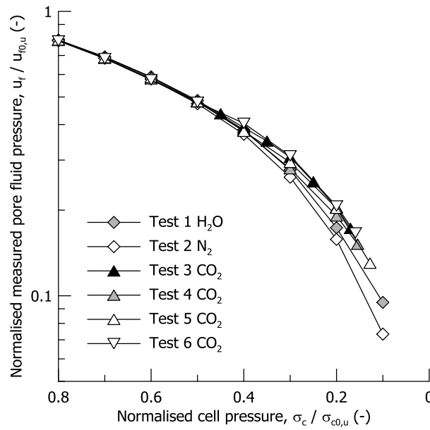
Fig. 3. Evolution of the measured pore fluid pressure during undrained unloading
