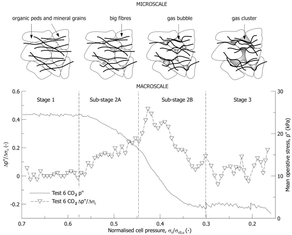
Fig. 11. Interpretation at the micro – macro scale of the gas exsolution process
