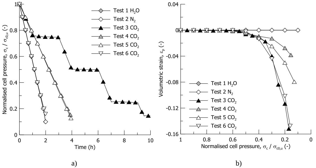
Fig. 2. Undrained unloading stage: (a) normalised cell pressure time sequence, (b) volumetric strains
