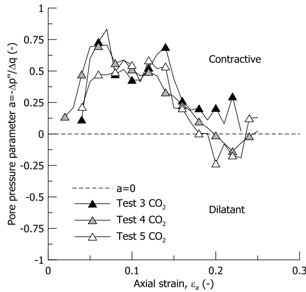
Fig. 14. Evolution of the pore pressure parameter a for the normally consolidated gassy samples during undrained shear
