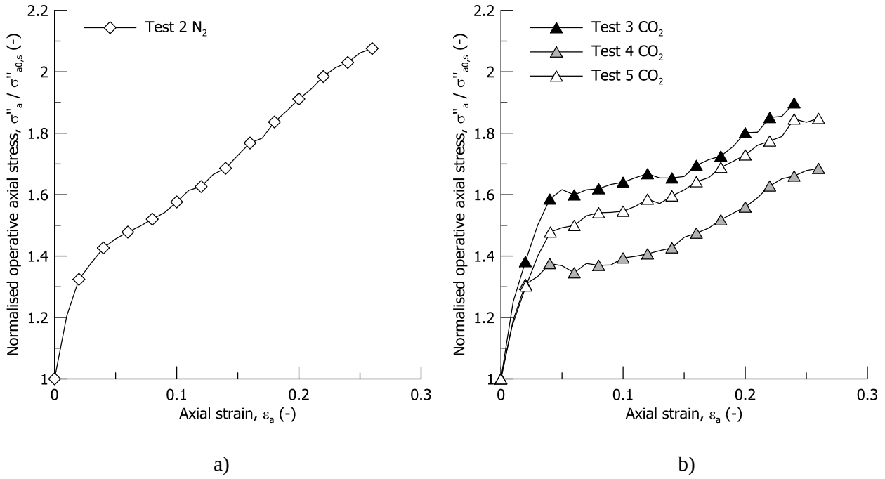
Fig. 15. Normalised operative axial stress-axial strain relationship: (a) fully saturated sample and (b) gassy samples
