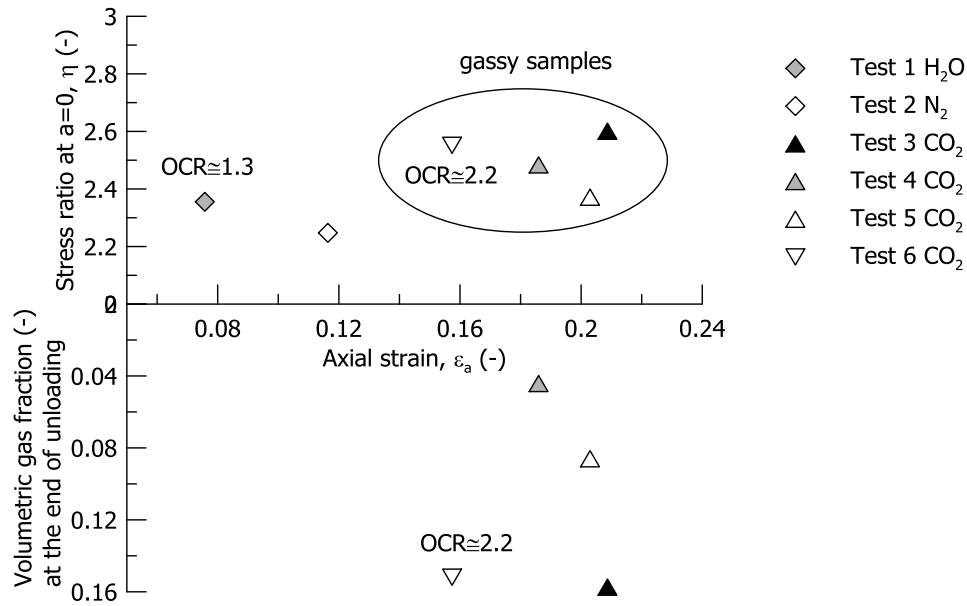
Fig. 16. Stress ratio plotted against axial strain at the onset of failure together with the volumetric gas fraction generated at the end of undrained unloading
