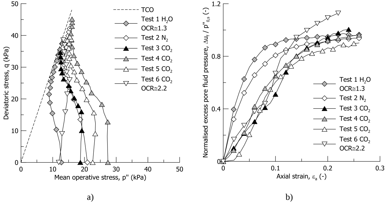
Fig. 4. Undrained shearing stage for fully saturated and gassy samples: (a) stress path, (b) excess pore fluid pressure versus axial strain
