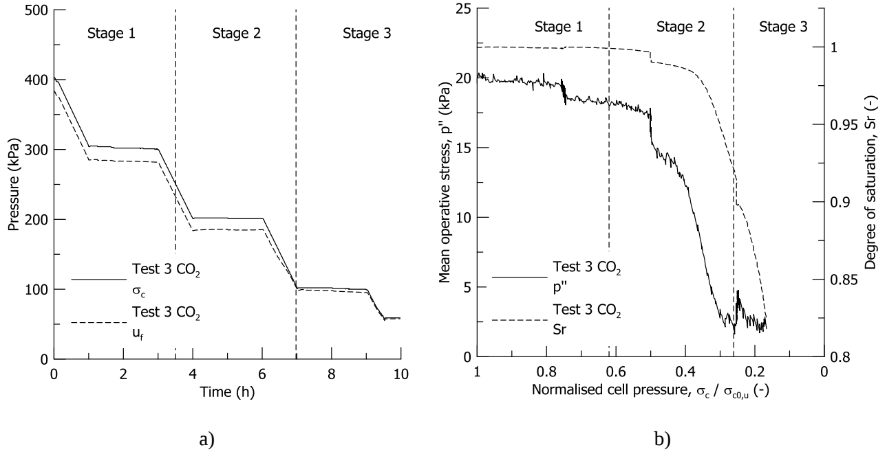
Fig. 7. Test 3 CO 2 : (a) cell pressure and pore fluid pressure evolution, (b) mean operative stress and degree of saturation evolution during undrained unloading
