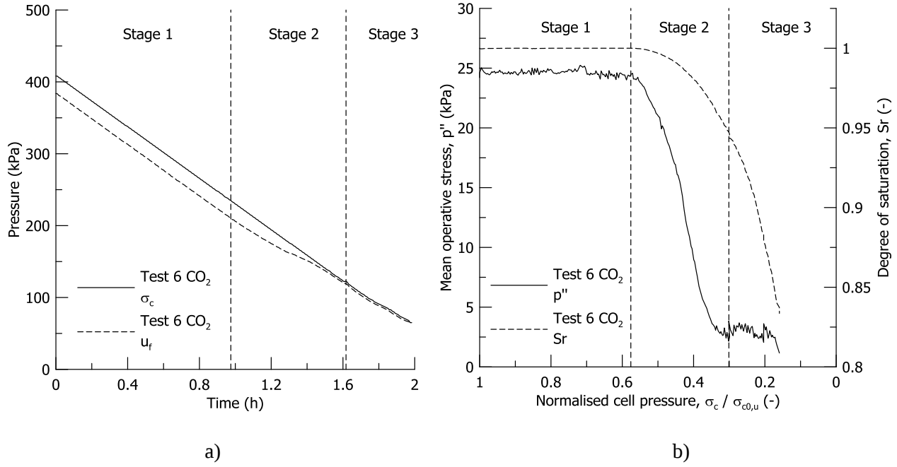
Fig. 9. Test 6 CO 2 : (a) cell pressure and pore fluid pressure evolution, (b) mean operative stress and degree of saturation evolution during undrained unloading
