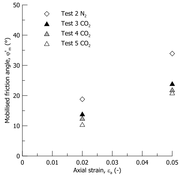
Fig. 17. Mobilised friction angle at axial strains of 0.02 and 0.05 for normally consolidated fully saturated and gassy samples
