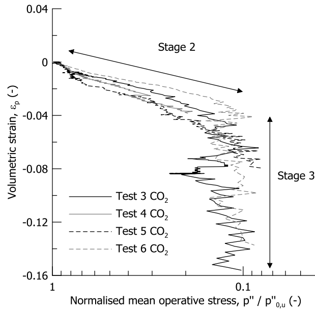
Fig. 12. Volumetric strains plotted against operative stress during undrained unloading for the gassy samples
