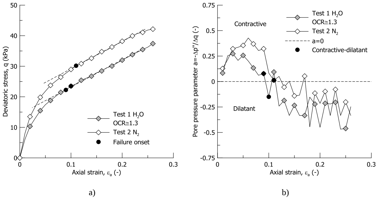
Fig. 13. Failure onset on the deviatoric stress-strain response (a) and (b) evolution of the pore pressure parameter a for fully saturated samples
