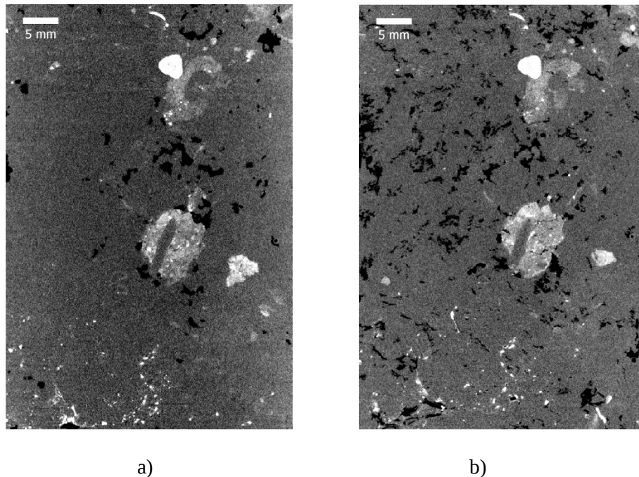
Fig. 5. Micro-CT scan of a gassy sample: (a) before gas exsolution; (b) after gas exsolution by undrained unloading. Black spots correspond to gas filled pores.
