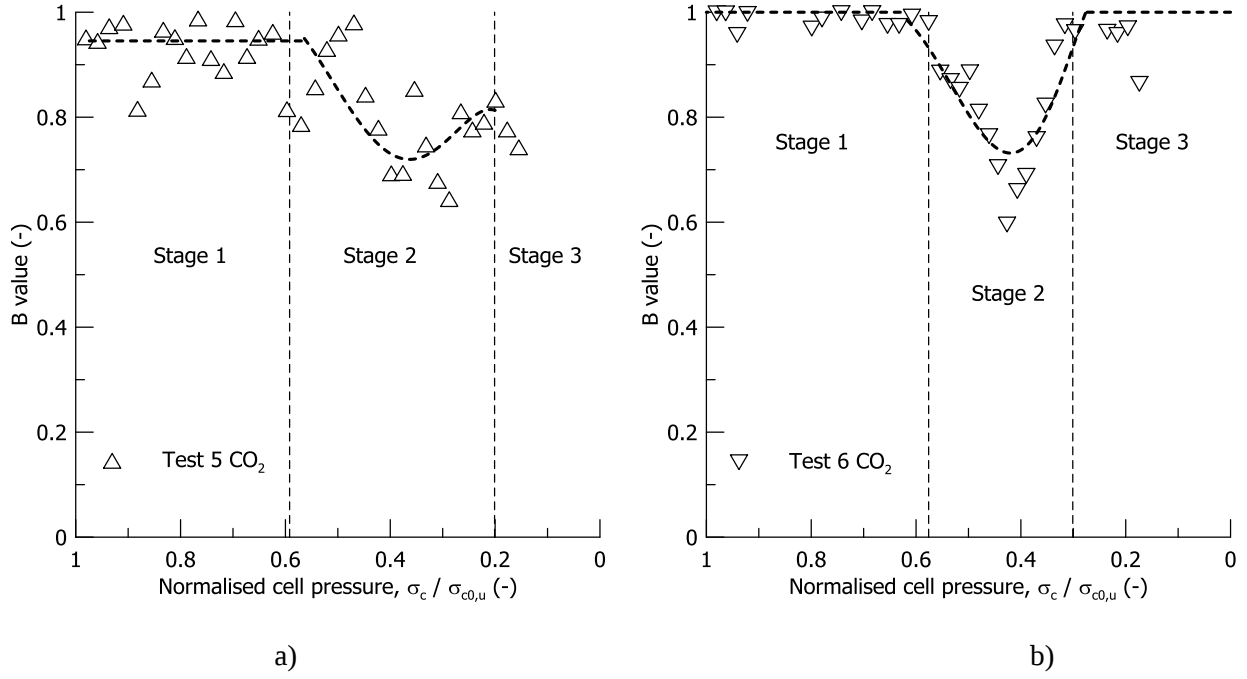
Fig. 10. Evolution of the B value during undrained unloading for two gassy samples: (a) Test 5 and (b) Test 6
