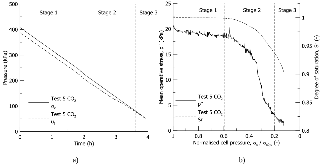
Fig. 8. Test 5 CO 2 : (a) cell pressure and pore fluid pressure evolution, (b) mean operative stress and degree of saturation evolution during undrained unloading
