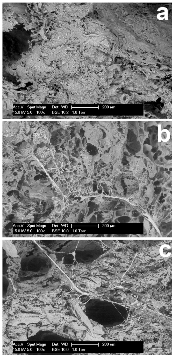
Fig. 2. ESEM analysis of freeze-dried structural EPS hydrogels with different metal ions at 100 times magnification. Freeze-dried gels were prepared with (a) magnesium, (b) calcium and (c) zinc.
