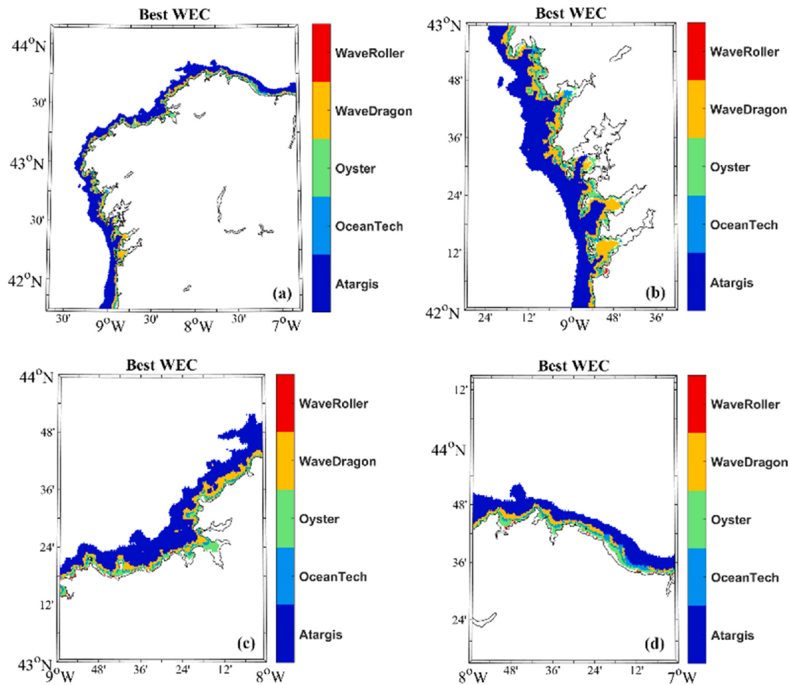
Fig. 6. The most profitable WEC for every location in the near future considering a CapEx = 1.5 M€/MW and r = 5\% (a) for the entire coastal area, (b) for the western coast, (c) for the northwestern coast and (d) for the northern coast of Galicia.
