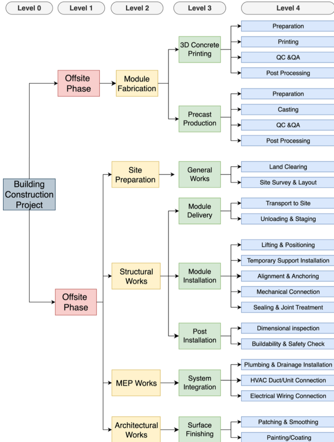
Figure 4: Four-Level WBS.
