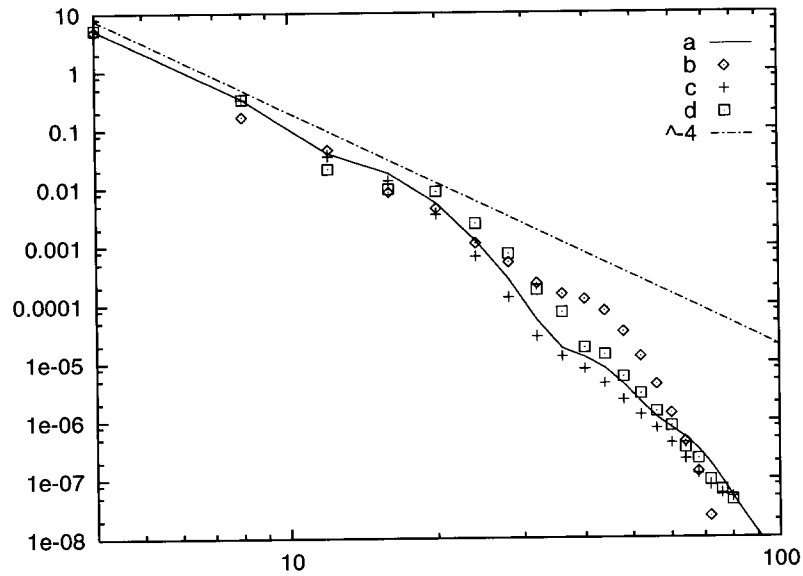
Figure 11. The one-dimensional energy spectra as defined by Equation (17)
