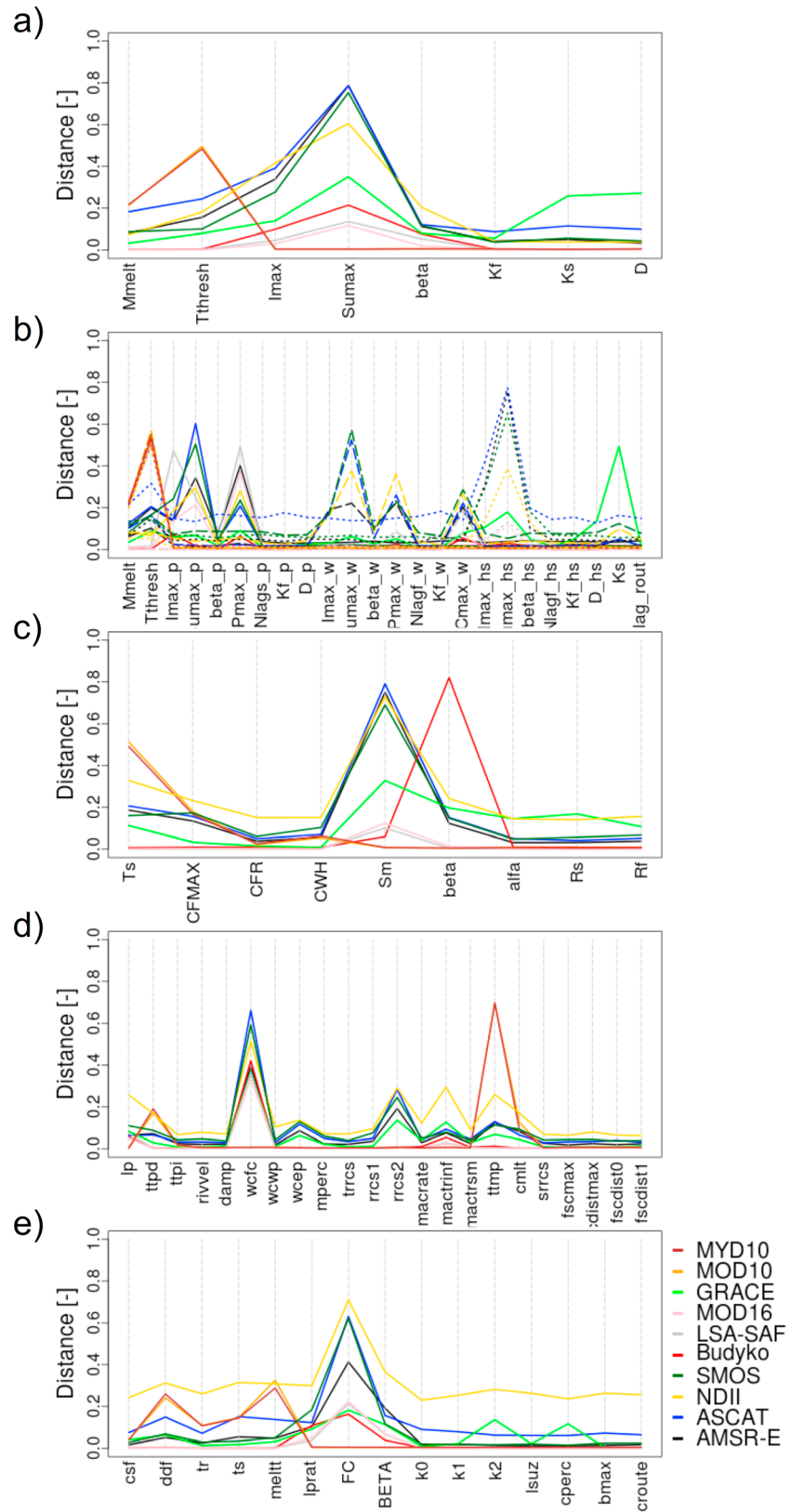
Figure 3. Sensitivity in average vertical distance between the empirical distribution curves of posterior and prior (uniform) parameter distributions for (a) FLEX, (b) FLEStopo, (c) HYMOD, (d) HYPE, and (e) TUW. Different colors indicate different products, with for FLEStopo a distinction per landscape class with plateau, wetland (dashed), and hillslope (dotted).
