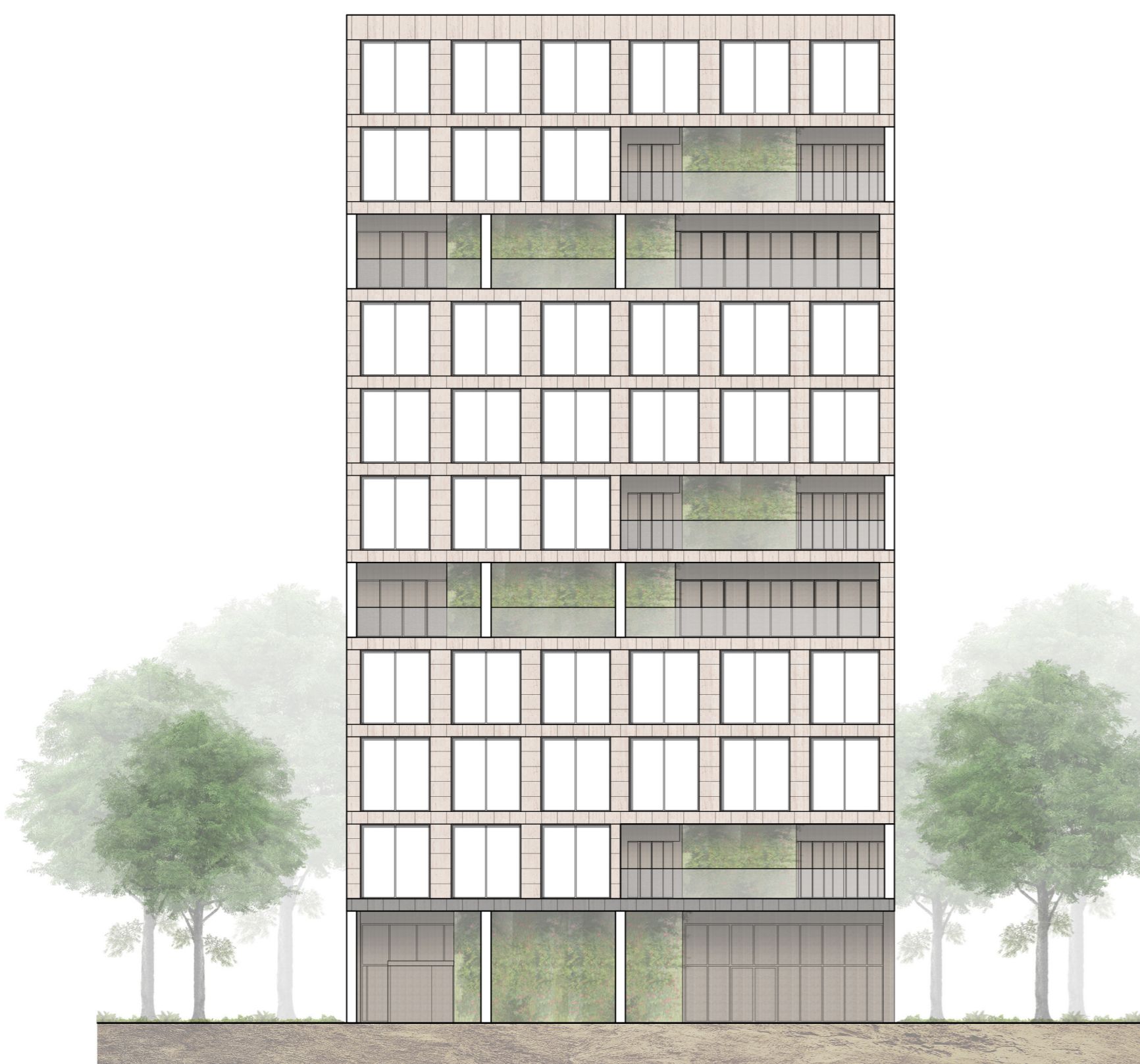
north elevation (1:200)
