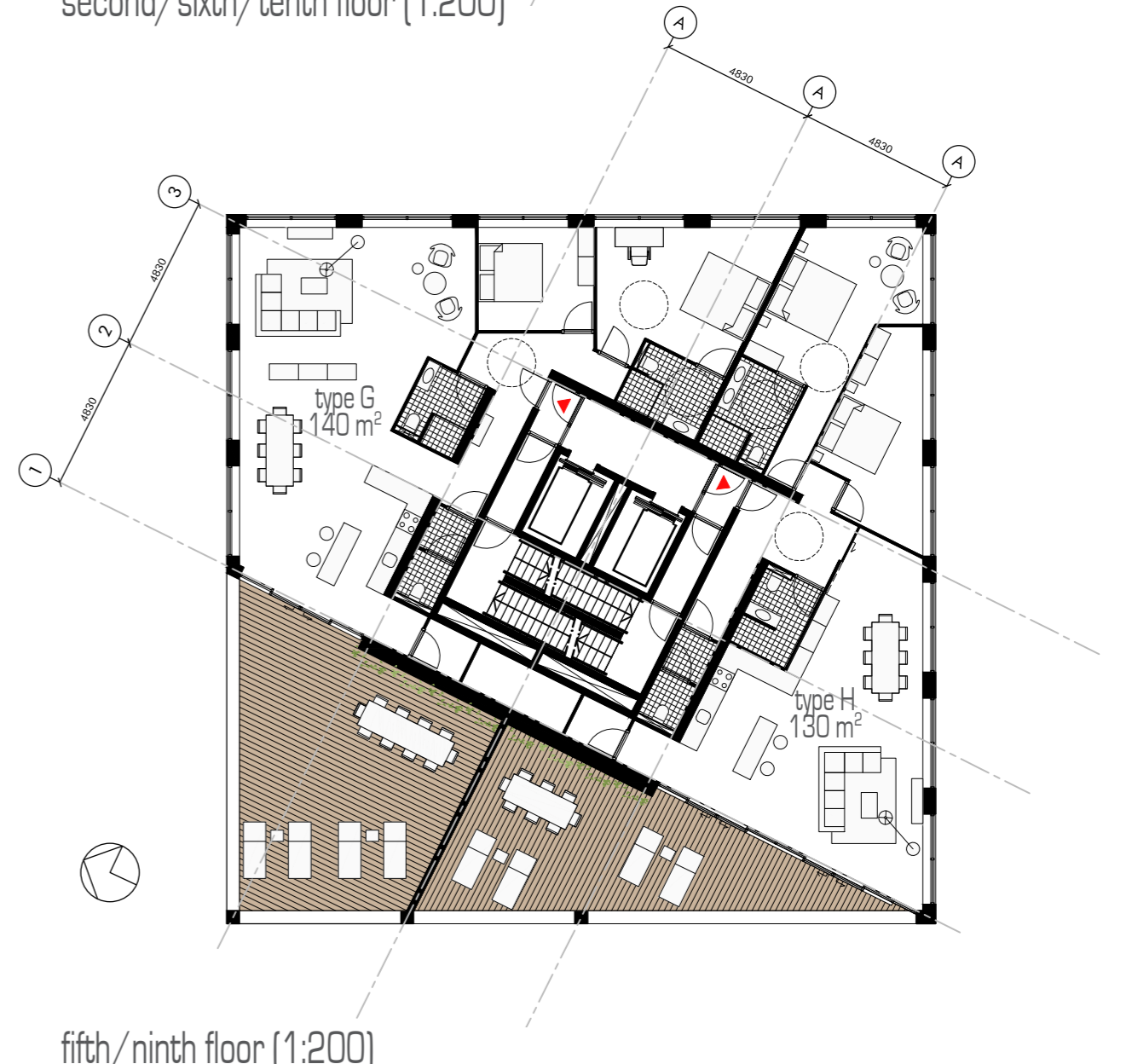
fifth/ninth floor (1:200)
