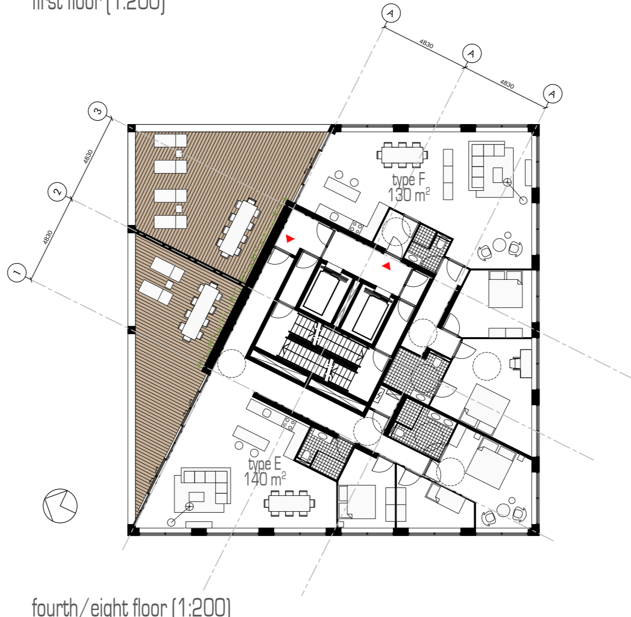
fourth/eighth floor (1:200)
