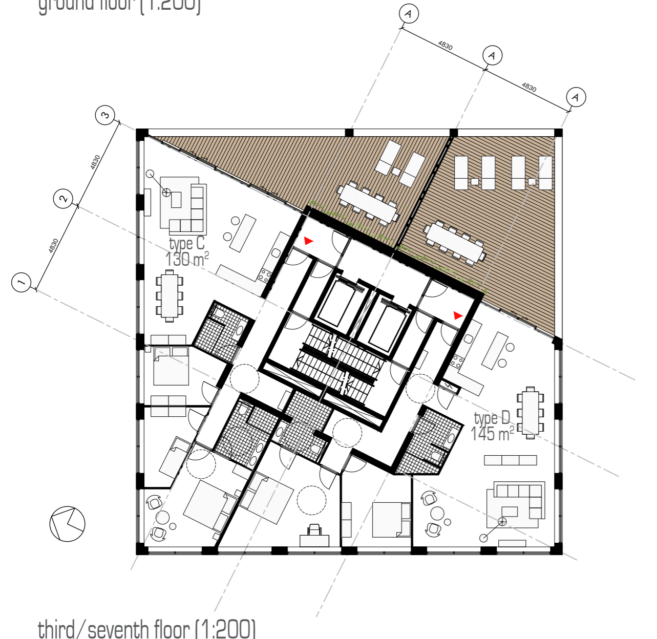
third/seventh floor (1:200)
