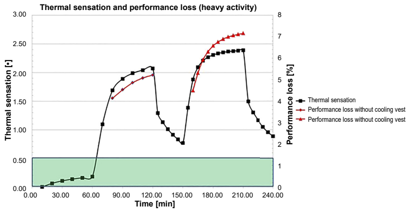
Figure 6. Thermal sensation and performance loss. Without a cooling vest. Heavy activity
