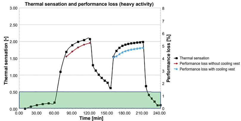
Figure 7. Thermal sensation and performance loss. Cooling vest donned after 150 min. Heavy activity
