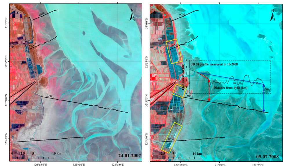
Figure 5. Satellite image of the JD 36 to 39 from Landsat 7 ETM on 24 January 2007 ( left panel ) and 5 July 2008 ( right panel ). The yellow box indicates the human interventions taking place between these two image times. The dash black box indicates the measured profile JD38 in October 2008, and the red and blue lines in the dash box are associated with two beach slope calculation methods.
