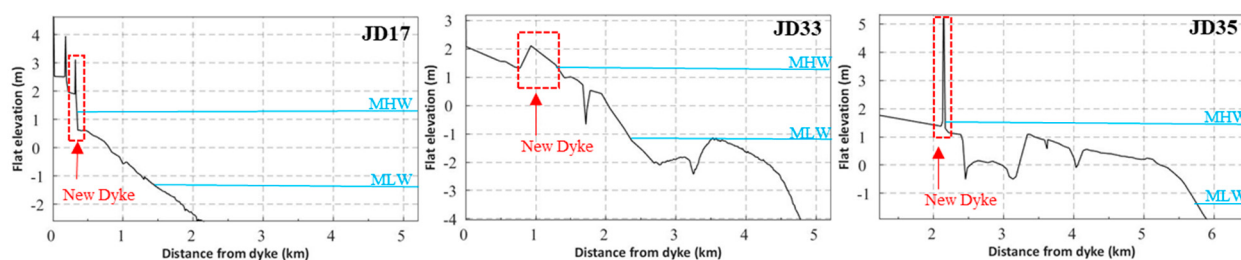
Figure 12. Zoom in on the bed elevation in front of and behind the newly built dykes (note that the scales of the three panels are not uniform).
