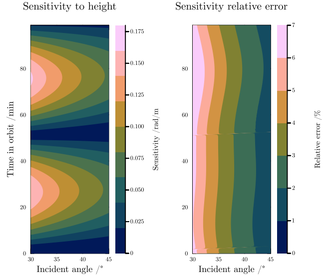
Fig. 9. Formation with a 650 m ascending node difference and a 125 m radial difference. Left panel: The sensitivity to height. Right panel: The relative error of the sensitivity calculated using the wavenumber method with respect to the conventional sensitivity expression.
