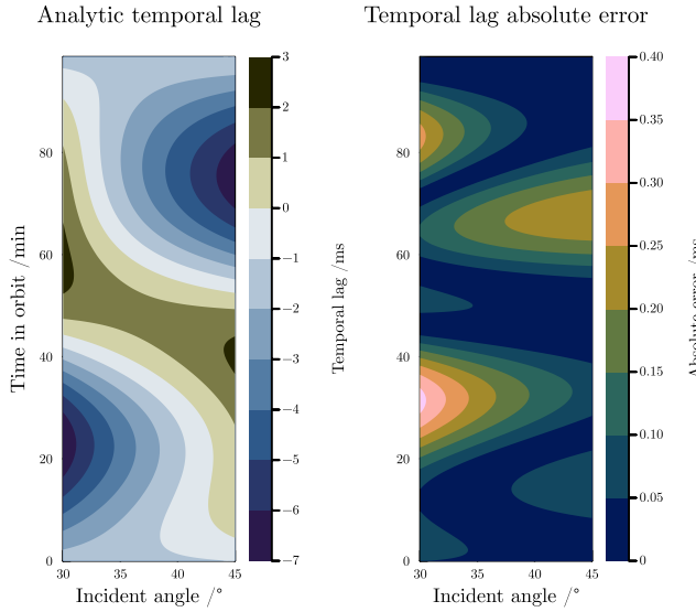
Fig. 8. Formation with a 650 m ascending node difference and a 125 m radial difference. Left panel: The temporal lag using the wavenumber method. Right panel: The absolute error between the temporal lag calculated spectrally and the temporal lag calculated using the geometric method.
