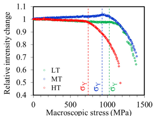
Fig. 5. Relative peak intensity of \{200\}\alpha' as a function of applied stress of LT, MT and HT specimens. Dashed lines indicate yielding of the material, \sigma_Y .
