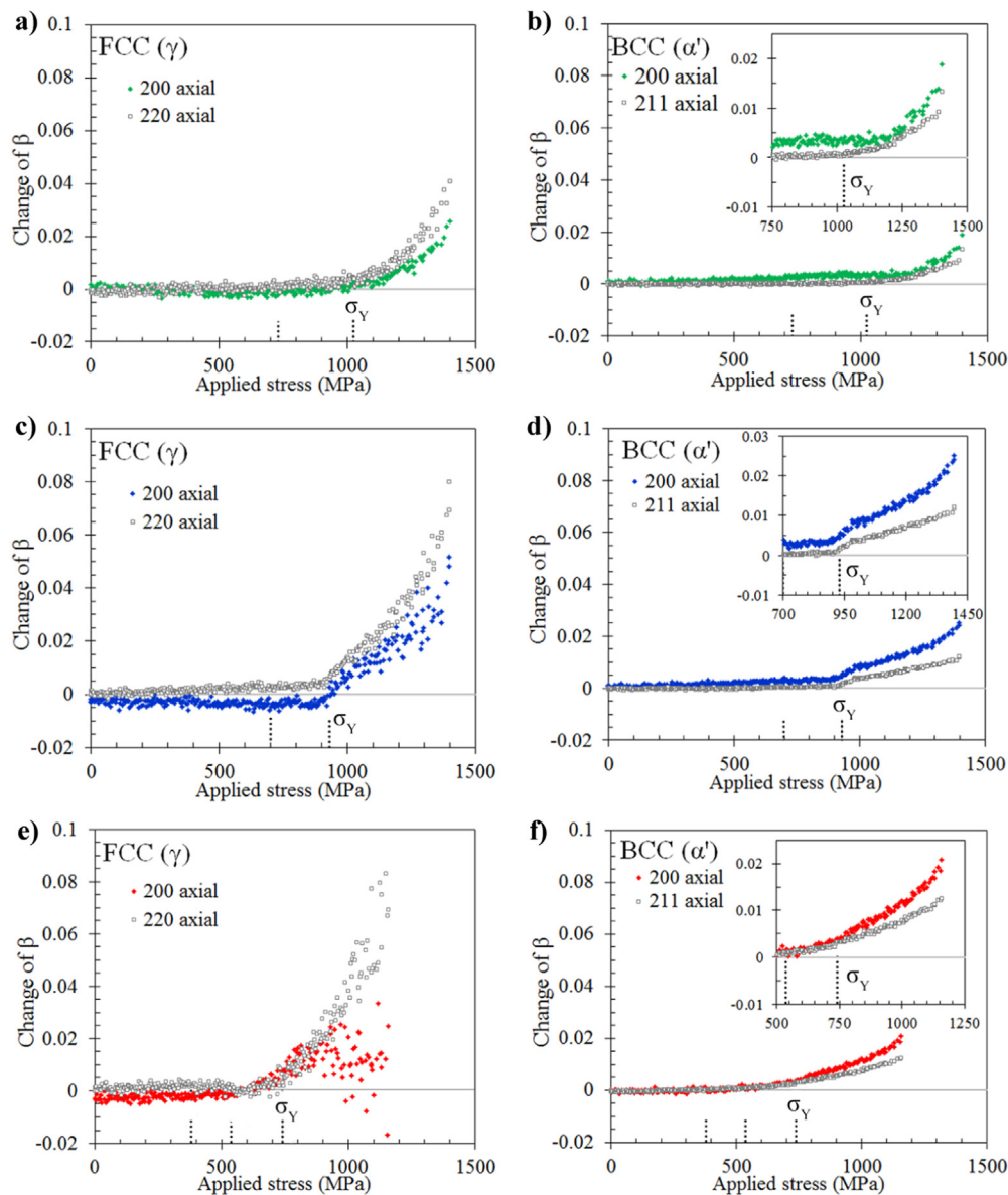
Fig. 4. Peak broadening evolution with applied stress of \{200\}\gamma and \{220\}\gamma , (a) LT, (c) MT and (e) HT specimens, and \{200\}\alpha' and \{211\}\alpha' in (b) LT, (d) MT and (f) HT. The dotted lines close to the axis delimit the anelastic region of the material and \sigma_Y the yielding of the material.
