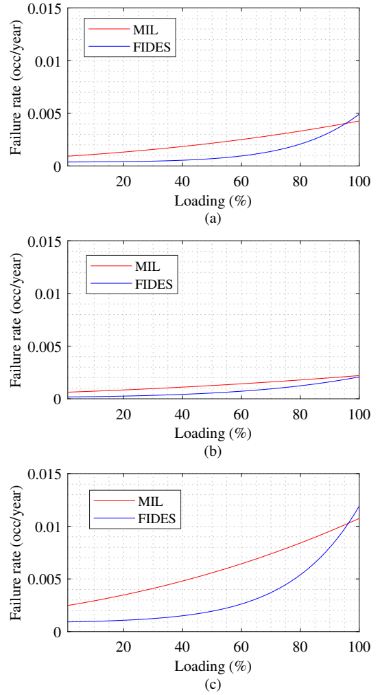
Fig. 2. Failure rate of (a) IGBT, (b) capacitor bank, and (c) SM with varying loading.
