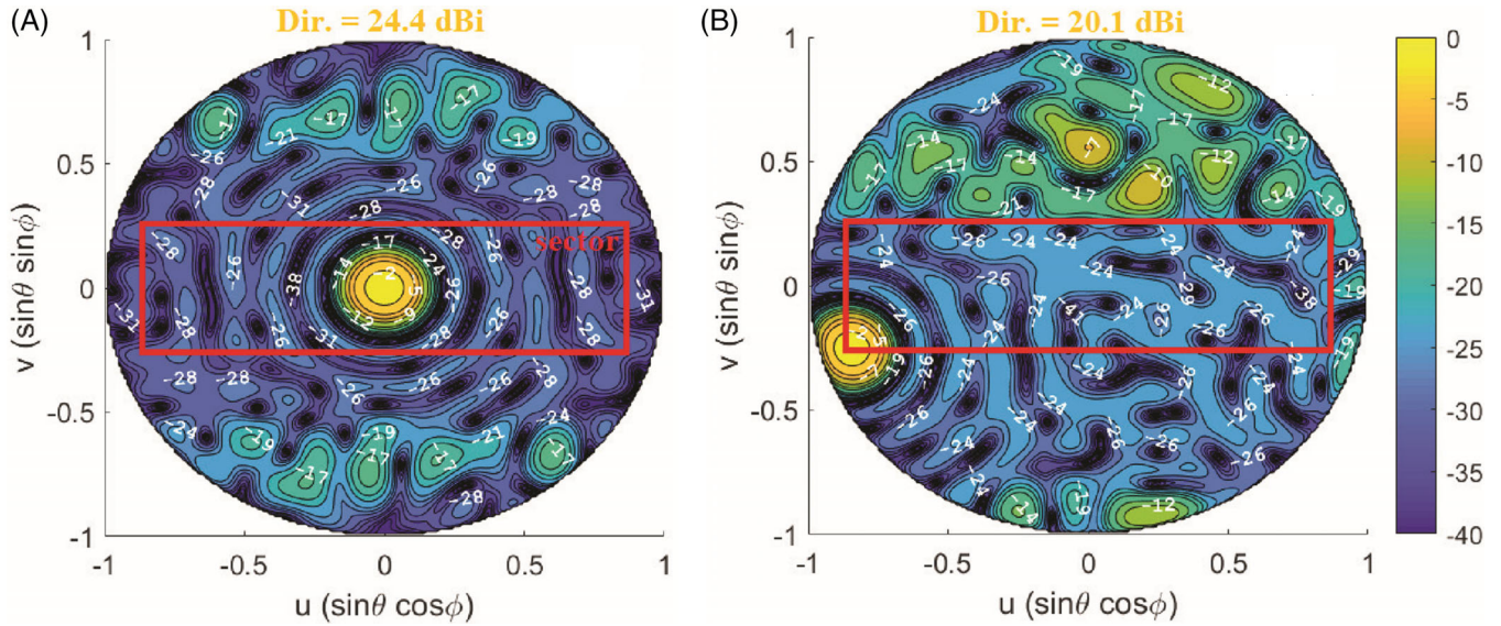
FIGURE 2 Multibeam radiation patterns (in dB, normalized with respect to the maximum beam directivity) of the optimized fully irregular 64-element array: (A) u_s = 0, v_s = 0 and (B) u_s = -\sin\pi/3, v_s = -\sin\pi/12 [Color figure can be viewed at wileyonlinelibrary.com ]
