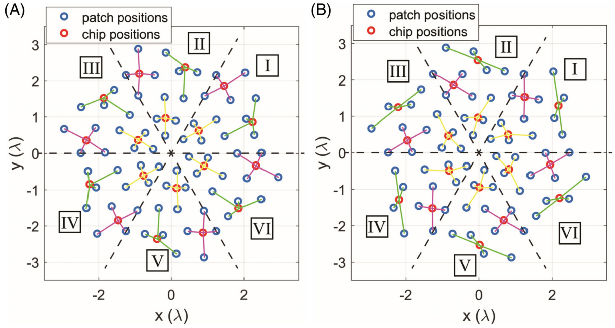
FIGURE 5 Sample suboptimal subarray clusters for the quasi-modular 72-element array: (A) option #1 and (B) option #2 [Color figure can be viewed at wileyonlinelibrary.com ]
