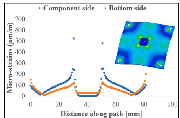
Fig. 6. FEM results showing the impact of strain gauge mounting location on measurements at board level.
