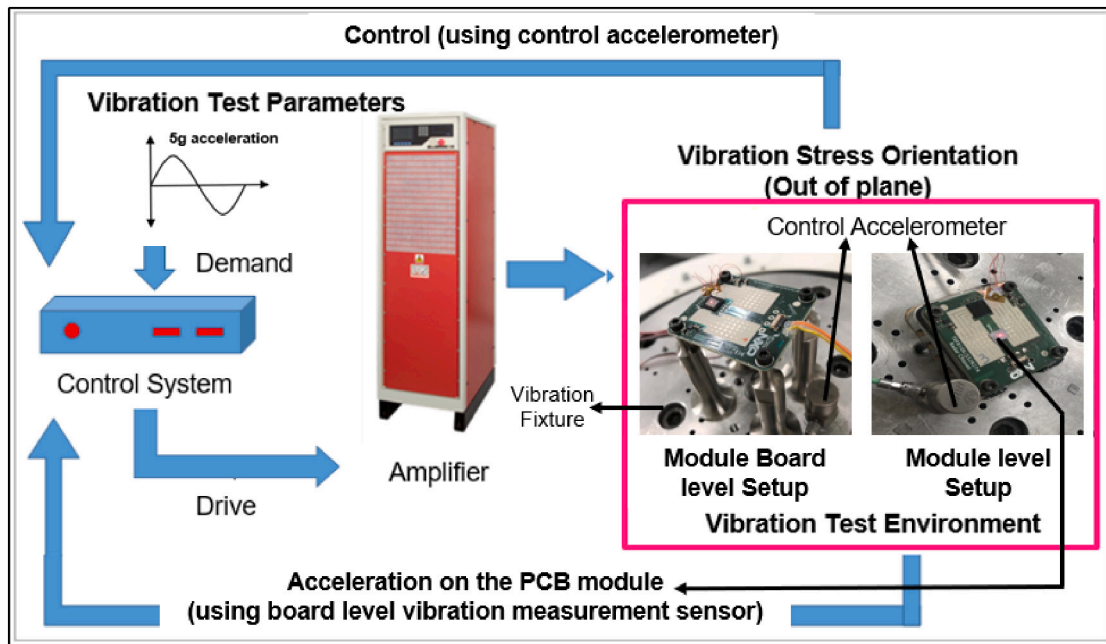
Fig. 3. Board Module, Module level vibration test setups.
