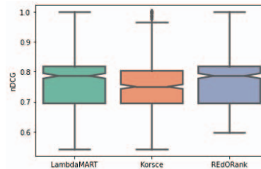
Fig. 1. NDCG@10 for different re-ranking models using RANKSET.
