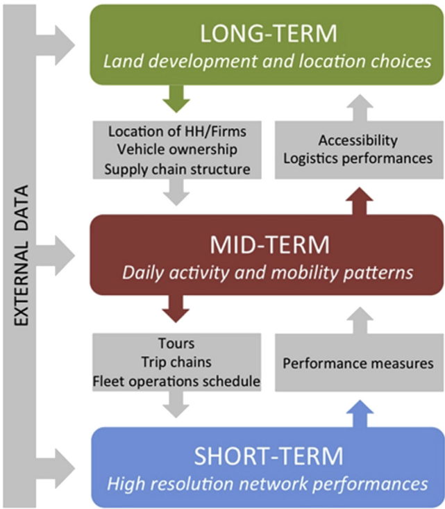
FIGURE 12.11 SimMobility framework (Adnan et al., 2016).
