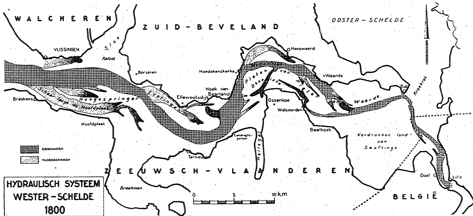
Fig. 26 System of ebb and flood channels in the West Scheldt in 1800. Badly developed part between Hoedekenskerke and Baalhoek.
