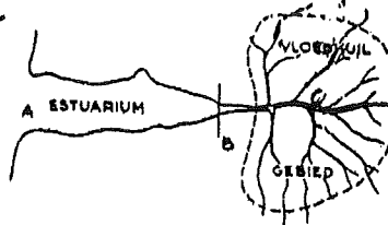
Fig. 7 A "flood depression" occurs in those areas where the tide (or stormtide) cannot enter fully, due to some bottle-neck. The floods become higher there, when dredging is done in the bottle-neck, or when the tidal fill of the area above the bottle-neck is diminished by reclamation works.
