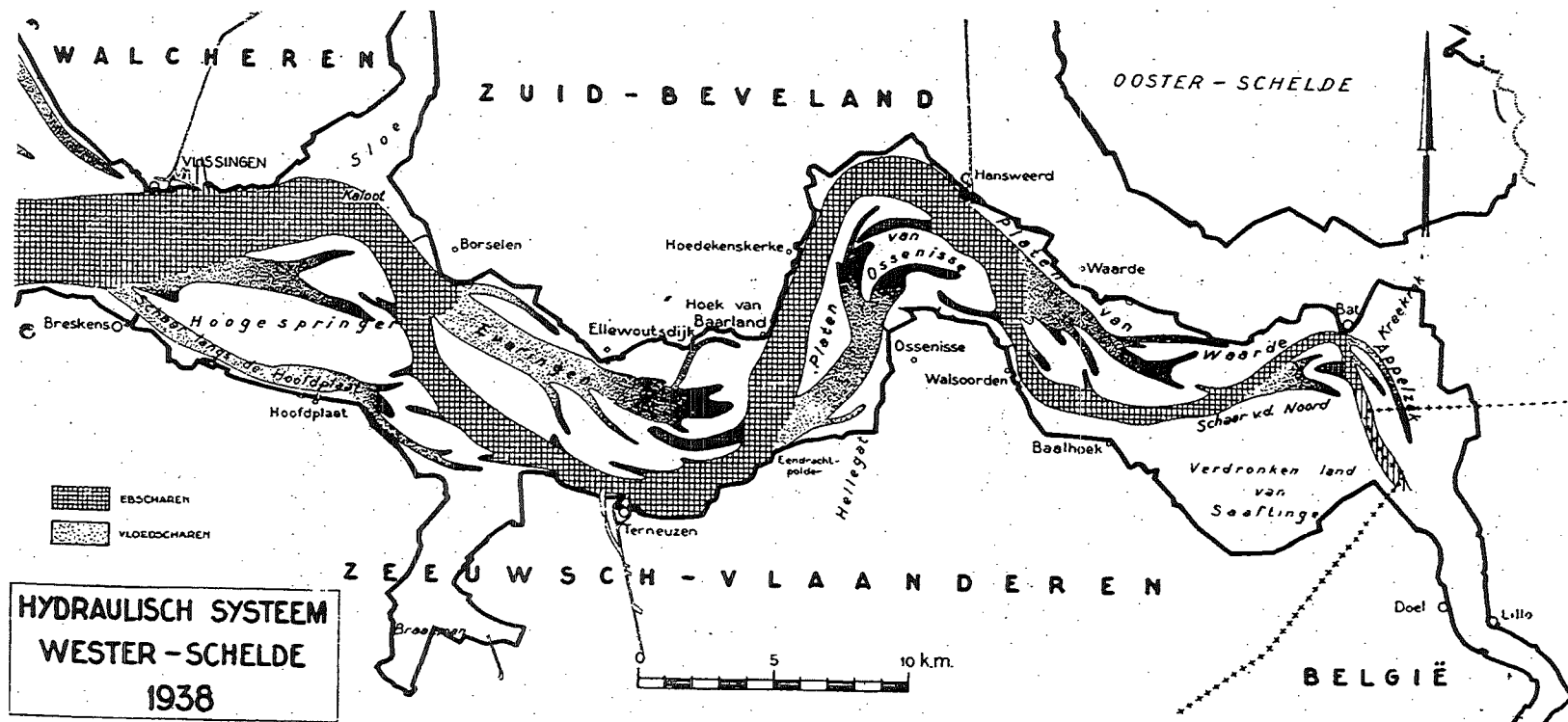
Fig. 28 System of ebb and flood channels in the West Scheldt in 1938. Well developed system at last.
