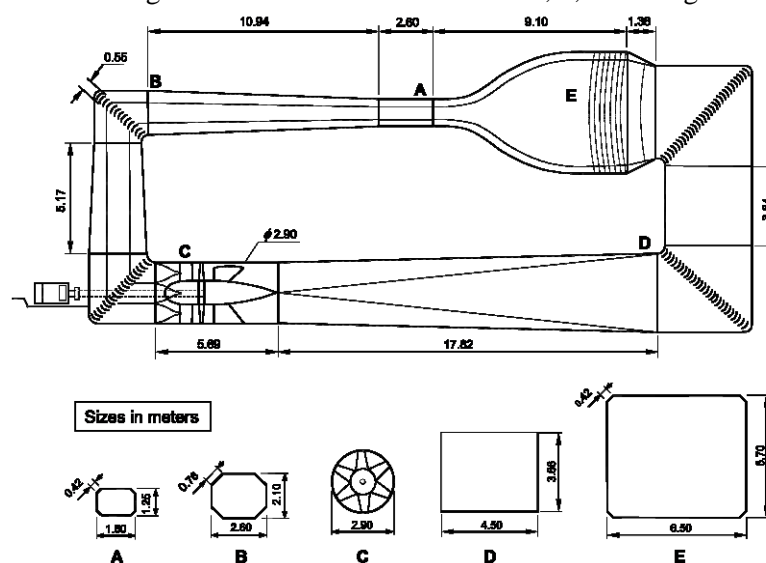
Figure 1. TU-Delft LSLT wind tunnel circuit lay out.
