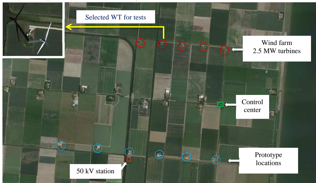
Figure 2. Overview of ECN Wind Turbine Test Site (EWTW).
