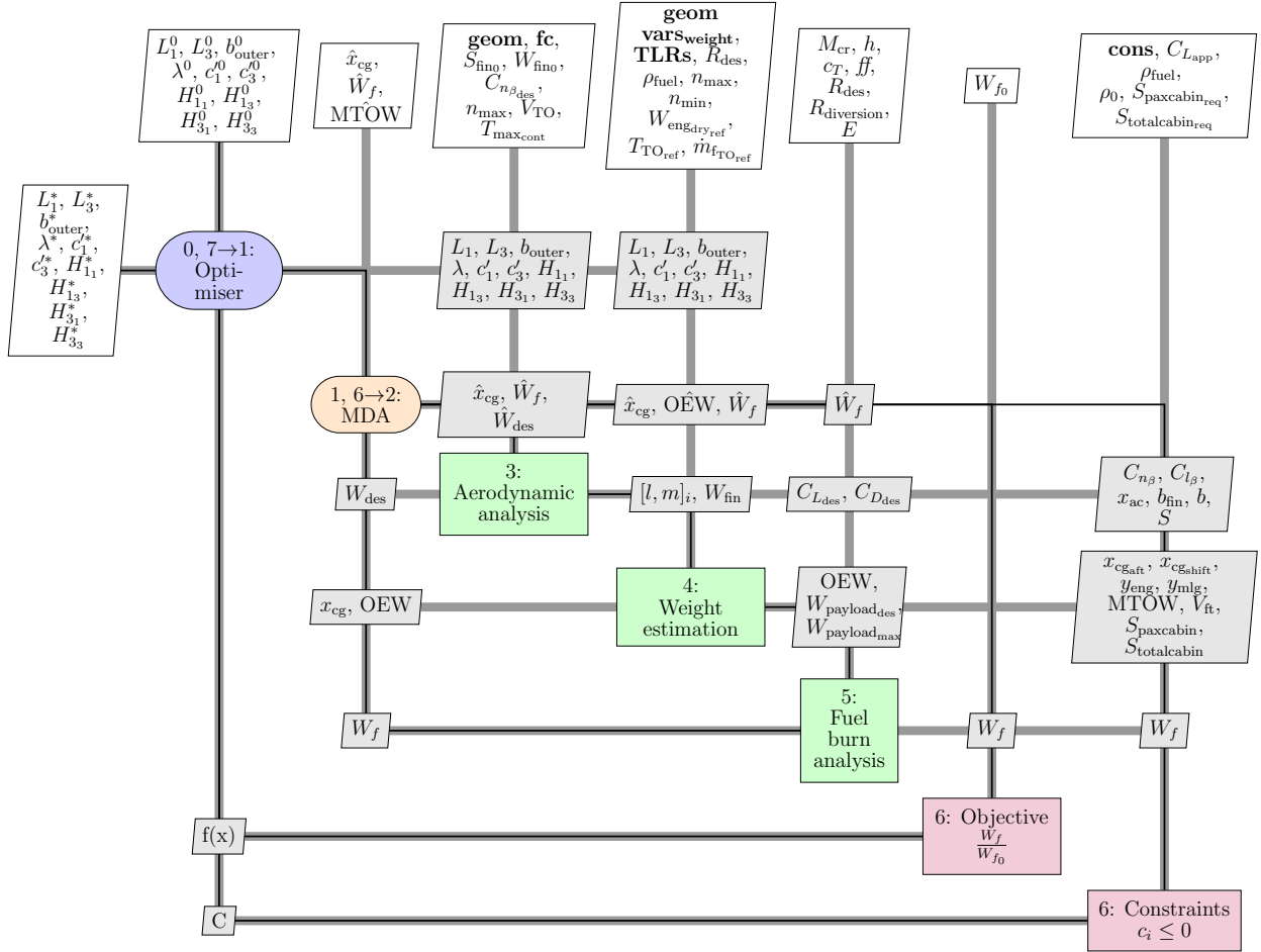
Fig. 3 Process flow of the design and optimization method for a single airplane. TLRs are top-level requirements provided in Table 6, cons are constraint values provided in Table 7, geom are fixed variables describing the Flying-V shape provided in Table 14, vars weight are inputs to the weight estimation model provided in Table 15 (see appendix) and fc are standard atmospheric conditions.
