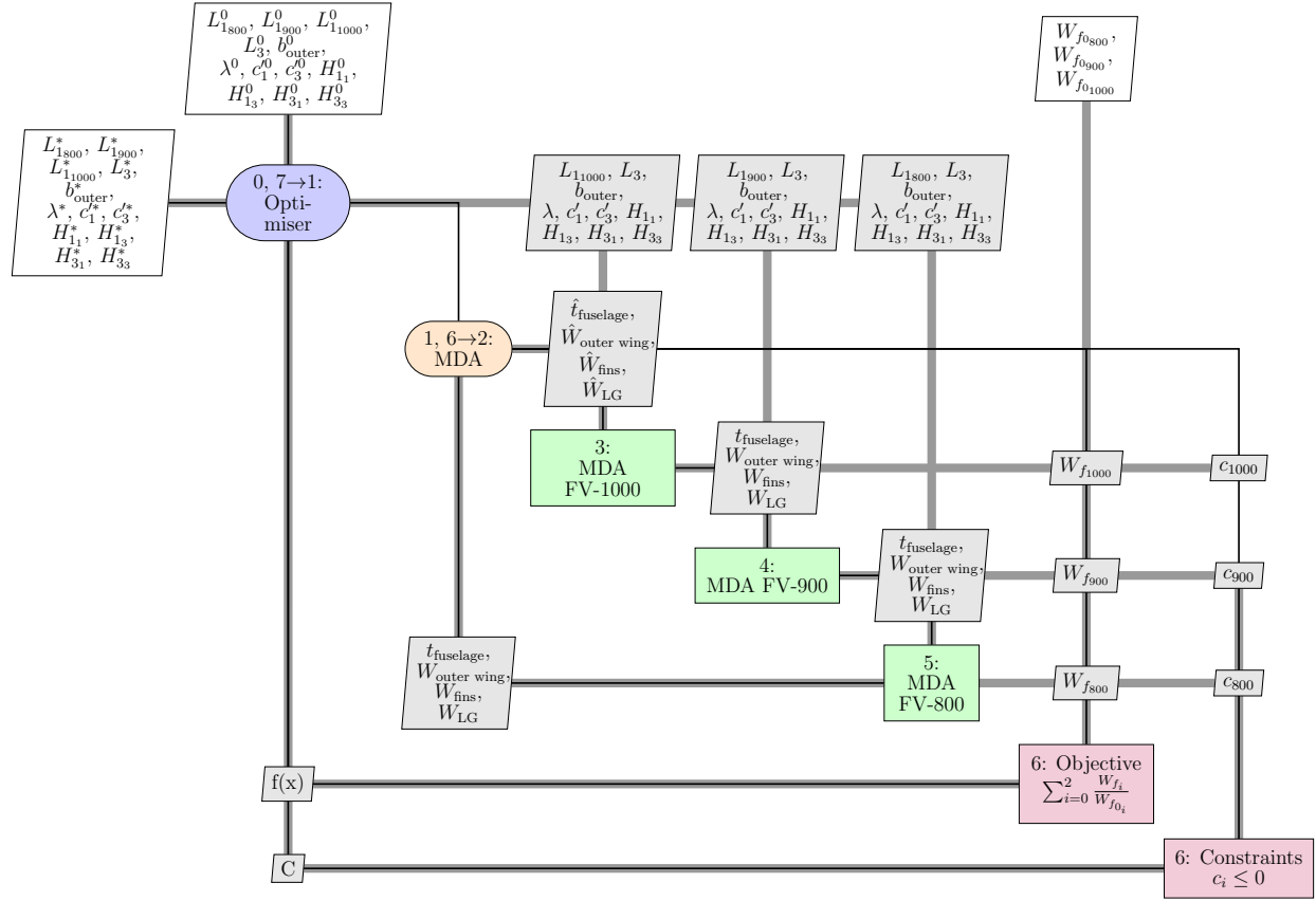
Fig. 4 Process flow of the aircraft family optimization method.
