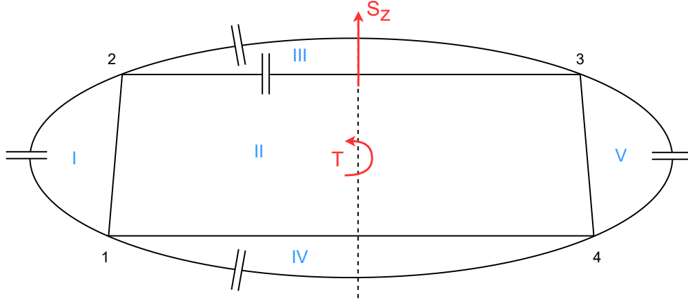
Fig. 13 Oval fuselage cross-section with numbered cells and vertices. Cuts to determine the open-section shear flow are indicated.
