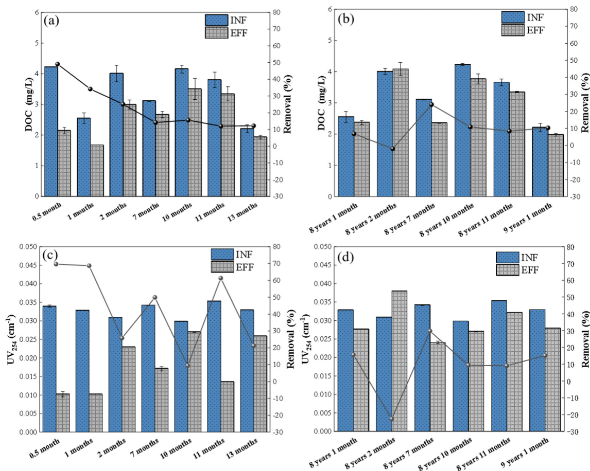
Fig. 1. Removal of DOC and \text{UV}_{254} by the new BAC (a, c) and the old BAC (b, d). The column stands for the concentration of DOC or \text{UV}_{254} . The line represents the removal percentage of DOC or \text{UV}_{254} .
