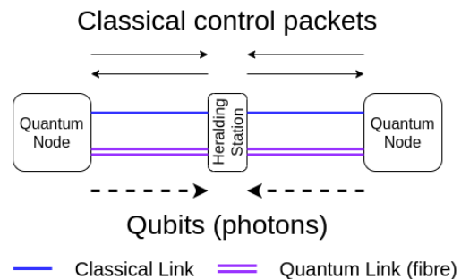
Figure 1: The heralding station upon simultaneous receipt of photons “heralds” the success or failure of an attempt.
