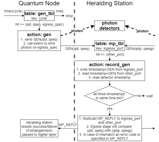
Figure 2: The node upon receipt of the timer pseudo-packet looks up its gen_tbl . A hit yields the parameters for the attempt and the node sends a photon and a GEN packet. The heralding station must wait for a GEN packet from both sides before it can send an MP_REPLY . The mp_tbl provides the other_port value as one heralding station can serve more than two nodes. For clarity not all pathways are shown.
