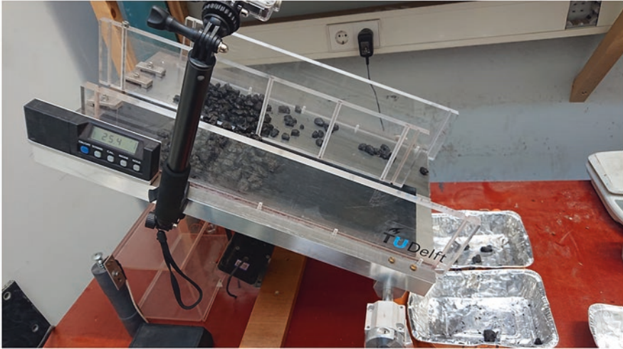
Fig. 4.20 Tilting table at the initiation of sliding/rolling of a set of nodules. (Doorn, 2022. Reprinted with permission)
