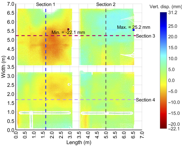
RANSAC (b)
