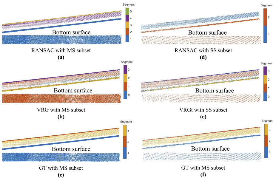
Figure 17. Point clouds of surfaces of the girder from various methods
