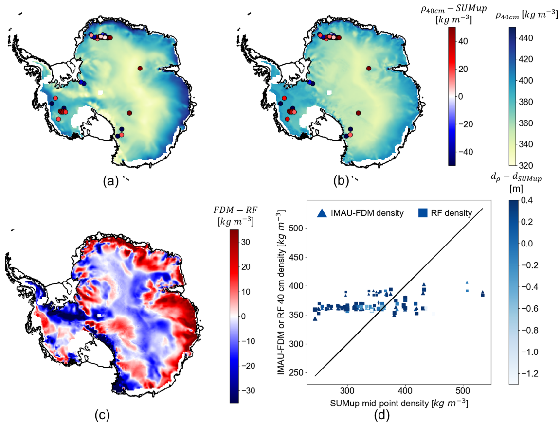
Figure 6. Maps of (a) temporally averaged IMAU-FDM 40 cm densities, (b) temporally averaged RF densities, and (c) the difference between averaged IMAU-FDM densities and RF densities (FDM – RF). Differences between the modelled or estimated densities and the SUMup densities are shown in scattered points in panels (a) and (b) as FDM-SUMup or RF-SUMup. Panels (a) and (b) share the same colour bar, in which blue–red shows the difference between the IMAU-FDM or RF densities and the SUMup densities ( \rho_{40\text{cm}} - \text{SUMup} ) and green–light blue shows the IMAU-FDM or RF densities ( \rho_{40\text{cm}} ). The coastline is from Depoorter et al. (2013). Panel (d) shows the relationship between IMAU-FDM or RF densities and SUMup densities. The sizes of the scattered points indicate the time difference between the SUMup measurements and the year 2020, and the colour shows the difference in depth between IMAU-FDM or RF measurements (both fixed at 40 cm) and SUMup measurements ( d_\rho - d_{\text{SUMup}} ).
