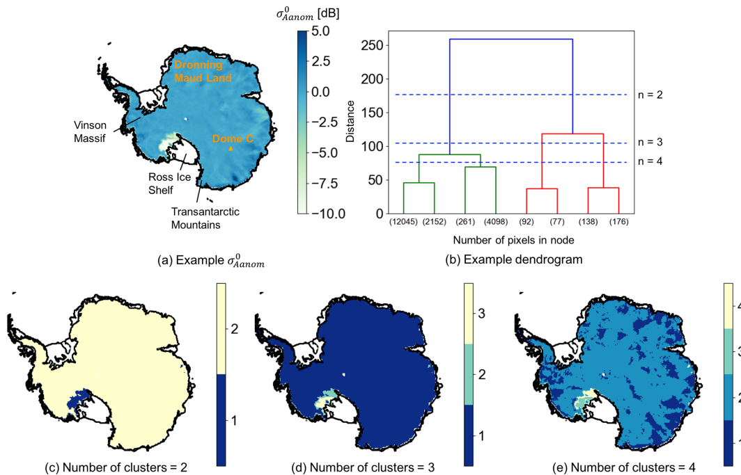
Figure 2. An example of the principle of hierarchical clustering. (a) Map of \sigma_{Anom}^0 acquired on 14 January 2016 following the melt event detected by Nicolas et al. (2017); (b) dendrogram obtained from panel (a), with low-hierarchy nodes simplified and n referring to the number of clusters; and (c)–(e) clustering results using different numbers of clusters. Several locations mentioned in this study are labelled in panel (a). The coastline is from Depoorter et al. (2013).
