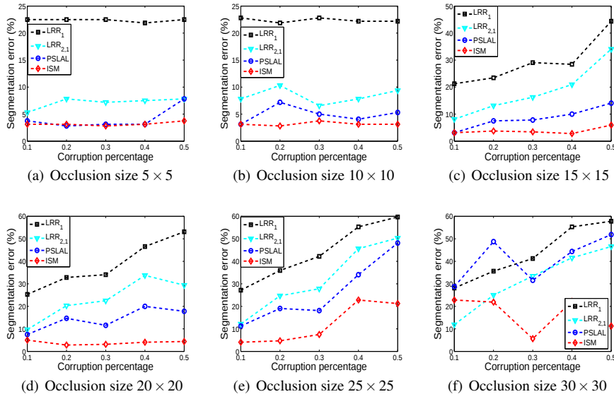
Fig. 5 Segmentation errors of different methods with various levels of occlusions.
