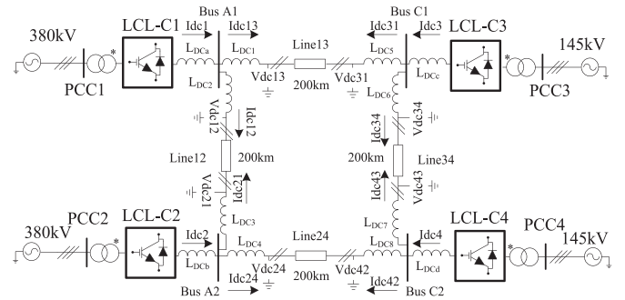
Fig. 1. A typical illustration of a terminal in an MTDC network.
