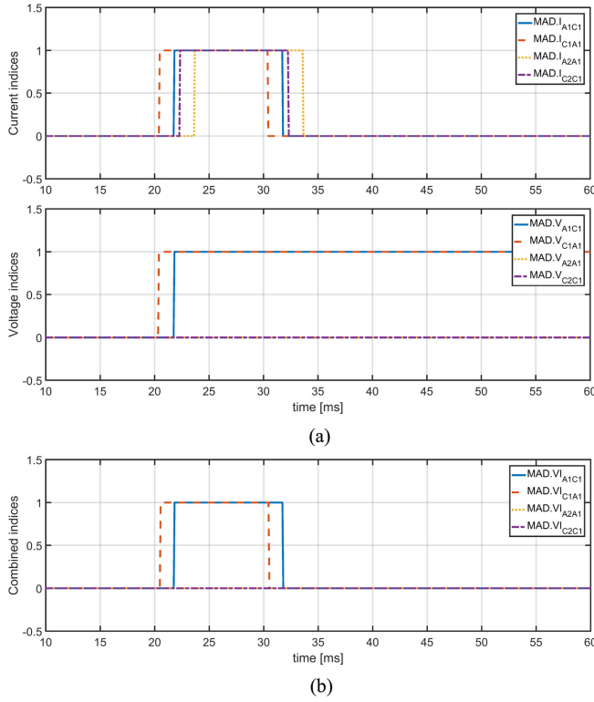
Fig. 9. Protection indices of the critical relays, (a) Current and voltage indices of critical relays, (b) Combined indices of critical relays.
