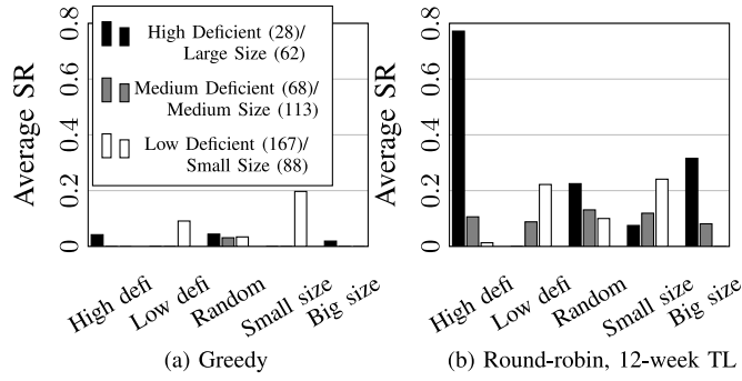
Fig. 9. Average SR based on different priority policies (numbers in parentheses are the members of each group).
