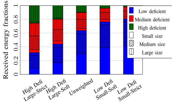
Fig. 10. Fraction of total energy received weekly by different groups - Weighted. High ratio between weights (strict): 1 \rightarrow 8 (step 1.0), Low ratio between weights (soft): 1 \rightarrow 3.33 (step 0.333)
