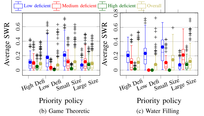
Fig. 12. Community social welfare ratio (yearly).
