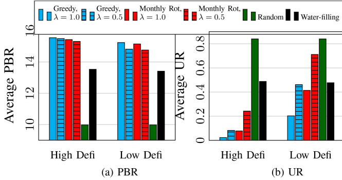
Fig. 11. Prosumer usage - Service diversity (week 38-49).
