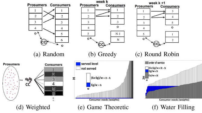
Fig. 4. Simple and Optimal Energy Allocation Strategies.
