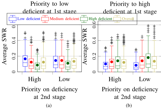
Fig. 13. Two stage energy sharing – GT for groups (1st stage), and WF individually (2nd stage).
