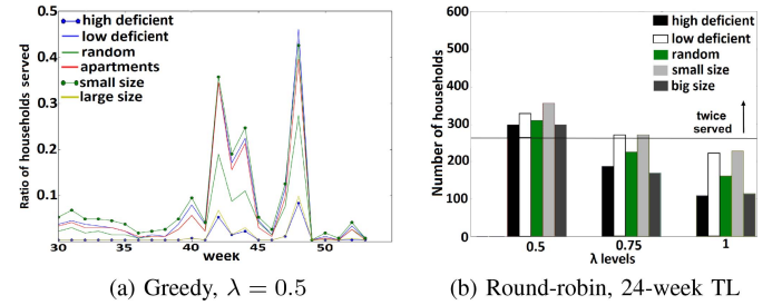
Fig. 8. Served households according to different priority policies and \lambda levels of service.
