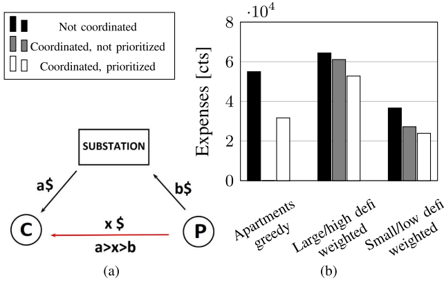
Fig. 14. (a) Cost schema; C: consumer, P: prosumer, (b) expenses reduction; pricing comparison from 10/13 to 10/26.
