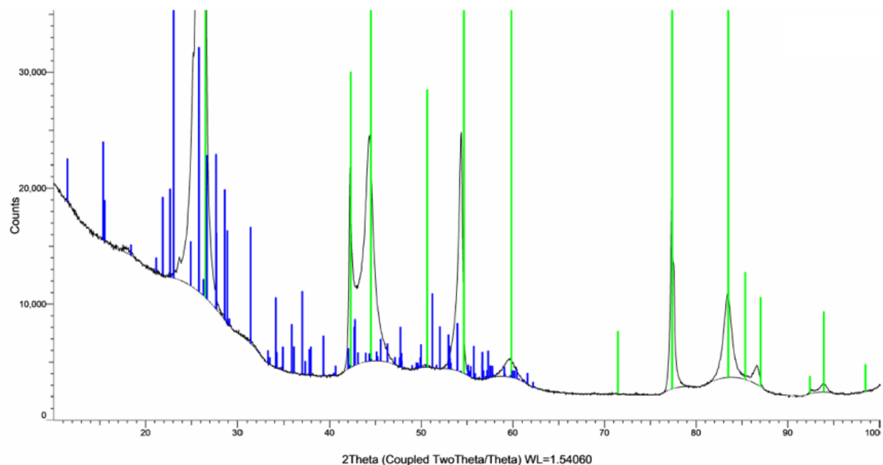
75 76 Figure C.2: XRD spectrum of the graphite plate at the end of experiment 2. The measurement was done 77 from 10 to 100 deg 2 theta, with steps of 0,05 deg, time/step 1s and xyz-sample stage. The measured 78 spectrum is shown by the black line. XRD spectrum of graphite is indicated in green; XRD spectrum of S 8 79 sulfur is indicated in blue.
