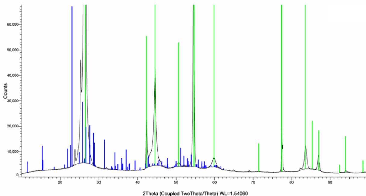
Figure C.1: XRD spectrum of graphite granules at end of experiment 2. The measurement was done from 10 to 100 deg 2 theta, with steps of 0,02 deg, time/step 3s. The measured spectrum is shown by the black line. XRD spectrum of graphite is indicated in green; XRD spectrum of S 8 sulfur is indicated in blue.
