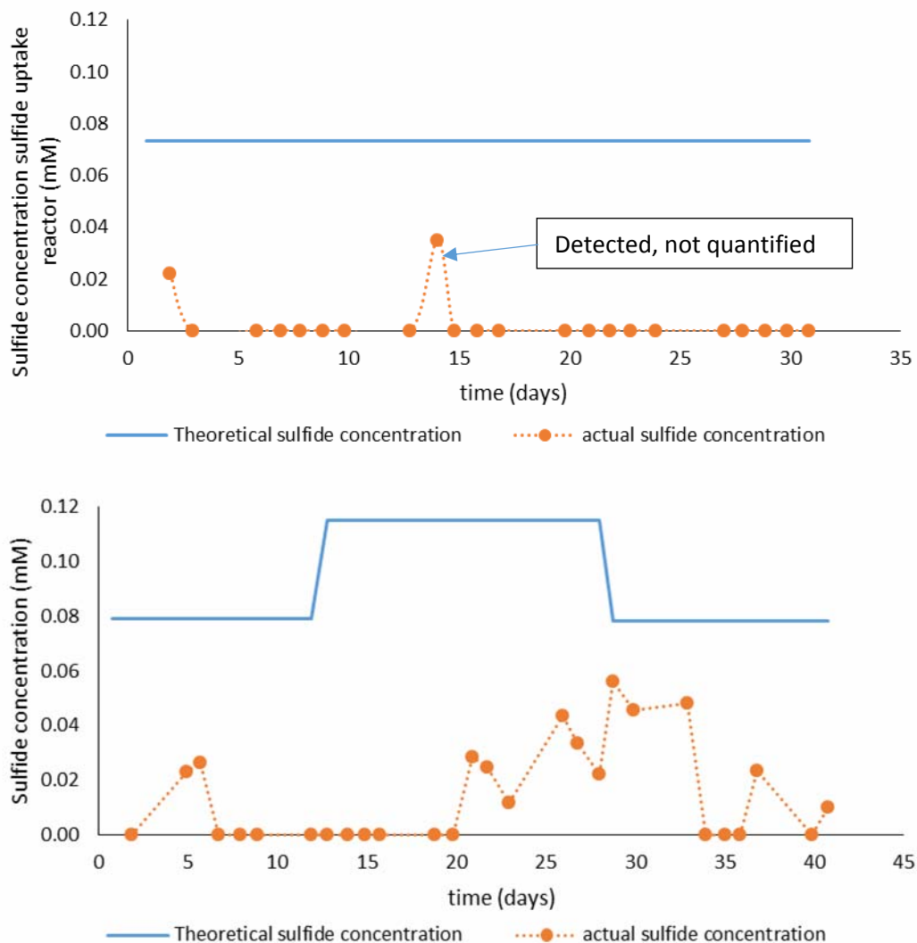
Figure D.1: The actual and measured sulfide concentrations in experiments 1 (top) and 2 (bottom). The blue line indicates the theoretical sulfide concentration in the sulfide uptake reactor, which is set by the sulfide dosing rate and the recirculation flow rate. The orange dots indicate the measured sulfide concentration in the sulfide uptake reactor.
