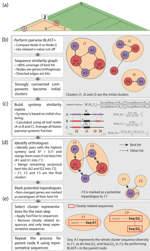
Fig. 1. Overview of the SynerClust algorithm. (a) Input phylogeny: example of a phylogenetic guide tree. SynerClust traverses the input phylogeny from the leaves to the root, iteratively computing sequence similarity and synteny, combining information from the children of each internal node. First, leaves B and C (children) are processed at internal node G (parent). Second, node G and leaf A are processed at internal node J. This second step is used as an example in the algorithm explanation below. (b) Initial clustering: for each parent orthogroup, representative sequences from child orthogroups are aligned (using MUSCLE [35]) and used to build a tree (using FastTree2 [21]). Groups of highly similar sequences are defined by applying a sequence similarity threshold (red boxes). The longest sequence is then selected as a representative for all other sequences within a set mutational distance. This is repeated by selecting additional representatives until all sequences are represented. (c) Calculation of syntentic fraction: a syntentic fraction for a specific orthogroup (orthogroup coloured in black) is calculated by dividing the number of shared neighbours within a 6 kb distance window (coloured in purple or red) by the total number of neighbours between two genomes (shared or unshared). For each cluster, a syntentic similarity matrix is built using the mean of all pairwise syntentic fractions. (d) Final clustering: final orthogroups for the current parent node are defined from the initial clusters by first looking for highly syntentic pairs, then for remaining pairs of reciprocal best hits. Child orthogroups that remain unmerged are marked as paralogues (potential inparalogues) of their best hit. At the next node, if they are still not part of an orthogroup, the mark is kept; otherwise it is removed. (e) Representative selection: for each parent orthogroup, representative sequences from child orthogroups are aligned (using MUSCLE [35]) and used to build a tree (using FastTree2 [21]). Groups of highly similar sequences are defined by applying a sequence similarity threshold (red boxes). The longest sequence is then selected as a representative for all other sequences within a set mutational distance. This is repeated by selecting additional representatives until all sequences are represented.
