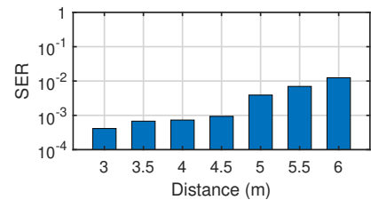
Figure 21: Symbol error rate of the side channel with multi-Level modulation.
