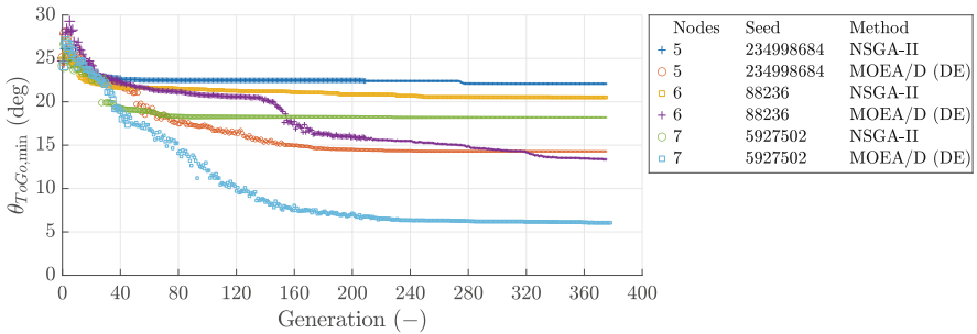
Fig. 9 Generational history of \theta_{ToGo,min} for an unconstrained single-objective coupled (ascent phase only), OFC-A, and initial population sourced from fitness vector ranking
