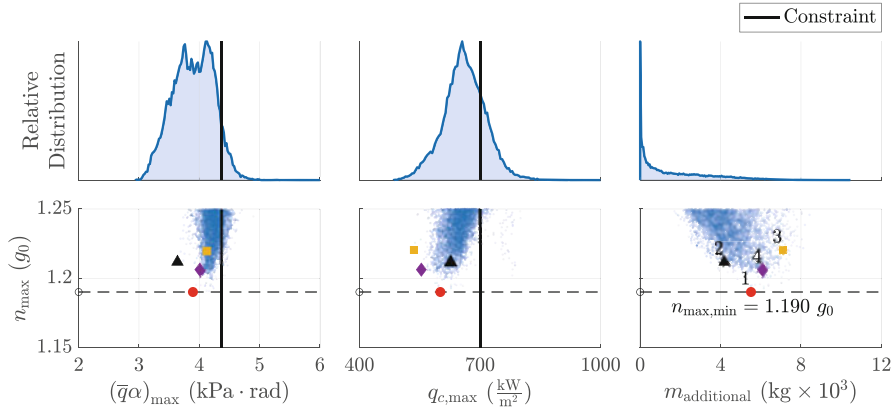
Fig. 14 Identification of sub-optimal and reference individuals used for localised global optimisation
