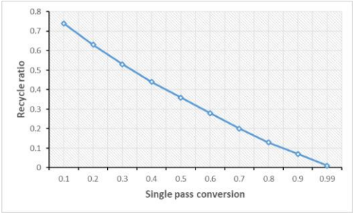
Figure 2 Single pass conversion vs Recycle ratio
