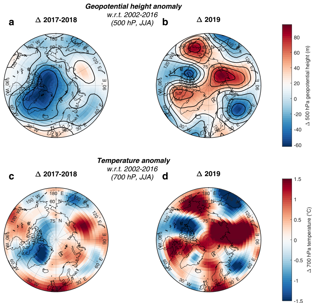
Fig. 4 Atmospheric conditions over the Arctic in summer for the low melt years of 2017 and 2018 and the strong melt year of 2019. Shown are summer mean (JJA) anomalies relative to 2002–2016. In 2017 and 2018, a 500 hPa geopotential height shows a pronounced low over Greenland, promoting below average (2002–2016), c temperatures at 700 hPa. In 2019, the pattern reversed with a higher, b 500 hPa geopotential height, accompanied by significantly warmer, d temperatures at 700 hPa in western Greenland. Thick black lines in a and b are contours of the anomaly of the 500 hPa geopotential height spaced at intervals of 20 m.
