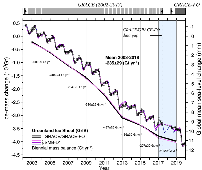
Fig. 1 Mass changes of the Greenland Ice Sheet between 2002 and 2019. Time series of mass change from the GRACE and GRACE-FO missions (black, with 2- \sigma error bars) and simulations using the regional climate models MARv3.10 30 (A; light violet) and RACMO2.3p2 31 (B; dark violet) and calibrated outflow measurements from feature tracking of optical and radar imagery (SMB-D*), updated from 32 (“Methods” section). The top bar indicates the availability of GRACE and GRACE-FO measurements, the vertical dashed lines frame the data gap between both missions. The blue shading covers the biennial period 2017–2018, which contains the GRACE/GRACE-FO data gap (dotted line). The monthly SMB-D* data shown for MARv3.10 (A*; dark blue) are linearly interpolated to match the GRACE/GRACE-FO measurement timeframes. Both datasets are fitted with a biennial piecewise linear trend (breakpoints on January 1st of each year), revealing accelerated mass losses until 2012, followed by a slowdown and particularly small loss during the years 2017 and 2018. Values denote biennial mass balances in \text{Gt yr}^{-1} .
