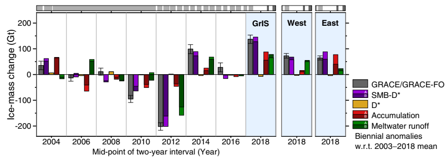
Fig. 2 Biennial mass balance anomalies and individual components for the Greenland Ice Sheet between 2003 and 2019. Shown are anomalies of the biennial mass balance from GRACE/GRACE-FO, with 2- \sigma error bars, and SMB-D* along with the components of accumulation, meltwater runoff and solid ice discharge (D*), with respect to their corresponding 2003–2018 mean values. For GRACE/GRACE-FO the 2003–2018 mean is -235 \pm 29 Gt year ^{-1} . Shown are results for MARv3.10 (A) and RACMO2.3p2 (B). The period 2017–2018 stands out with the most positive mass loss anomaly of +137 \pm 25 Gt year ^{-1} , caused in equal parts by enhanced snowfall and reduced meltwater runoff in the eastern and western drainage basins, respectively 37 . The top bar indicates the availability of GRACE and GRACE-FO measurements.
