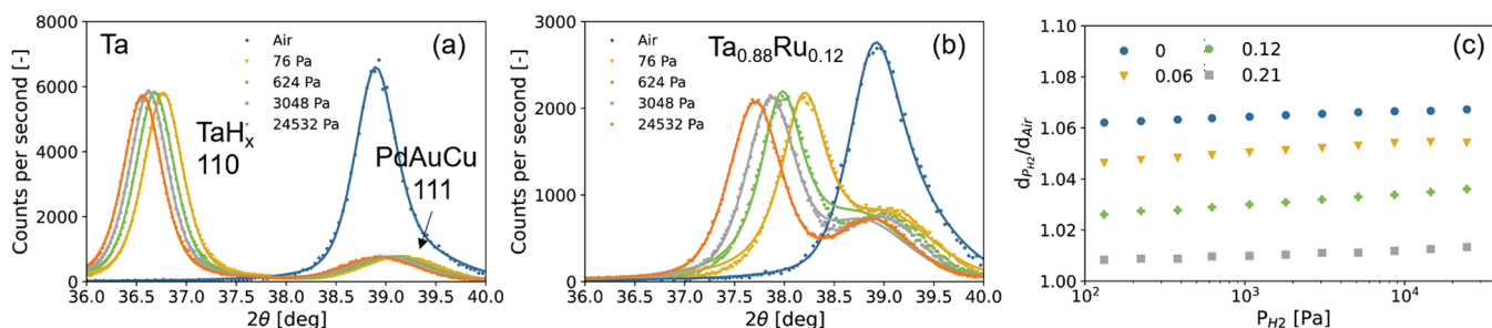
Figure 2. In situ XRD results of the 40 nm \text{Ta}_{1-y}\text{Ru}_y thin films with a 4 nm Ti adhesion layer and capped with a 10 nm \text{Pd}_{0.6}\text{Au}_{0.35}\text{Cu}_{0.05} at T = 25^\circ\text{C} . (a, b) Diffraction patterns (Cu K\alpha , \lambda = 0.154 nm) of the \text{Ta}_{1-y}\text{Ru}_y thin films with (a) y = 0 and (b) y = 0.12 measured for the hydrogen pressures indicated in the legend and for decreasing pressure steps. The continuous lines represent fits of two pseudo-Voigt functions to the experimental data. (c) Hydrogen pressure dependence of the expansion of the d_{110} -spacing in \text{Ta}_{1-y}\text{Ru}_y relative to the unloaded state in air.
