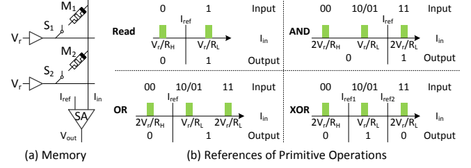
Fig. 4. Main idea of Scouting Logic [13].
