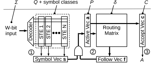
Fig. 9. Architecture of RRAM-AP [25].
