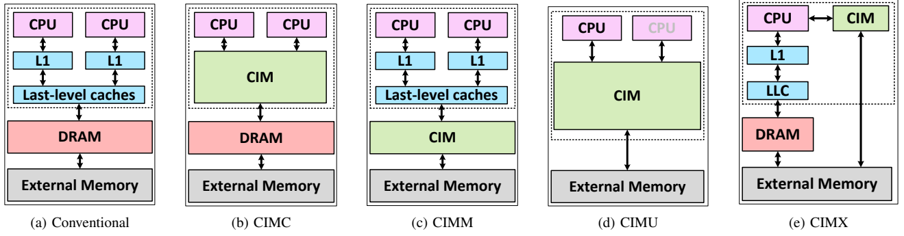
Fig. 3. Conventional architecture and potential CIM architectures.
