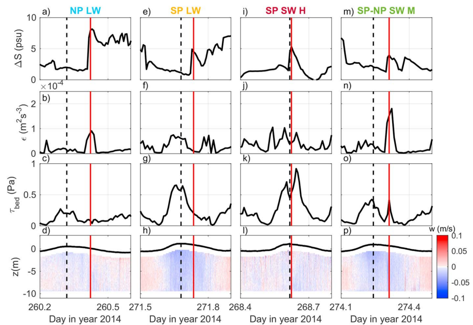
Figure 10. Near bed properties for different periods. The vertical axes represents salinity difference bottom-top (psu), dissipation ( \text{m}^2/\text{s}^3 ), bed stress (Pa), and depth (m). The horizontal axes represent different periods: NP LW, SP LW, SP SW H, and SP-NP SW M. The colorbar in the fourth row represents vertical velocity (m/s) based on 1-min averaged ADCP data, where positive is upwards and negative downwards. The dashed black lines indicate HW and the solid red lines indicate the front.
