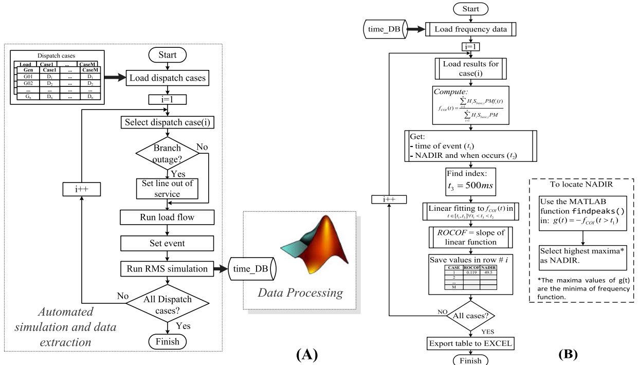
FIGURE 13. A) Procedure for automated simulation and data extraction by combining PowerFactory, Python, and Excel. time_DB stands for a database of time responses of system variables; B) procedure for data processing of frequency response and calculation of ROCOF and NADIR by using Matlab and Microsoft Excel.
