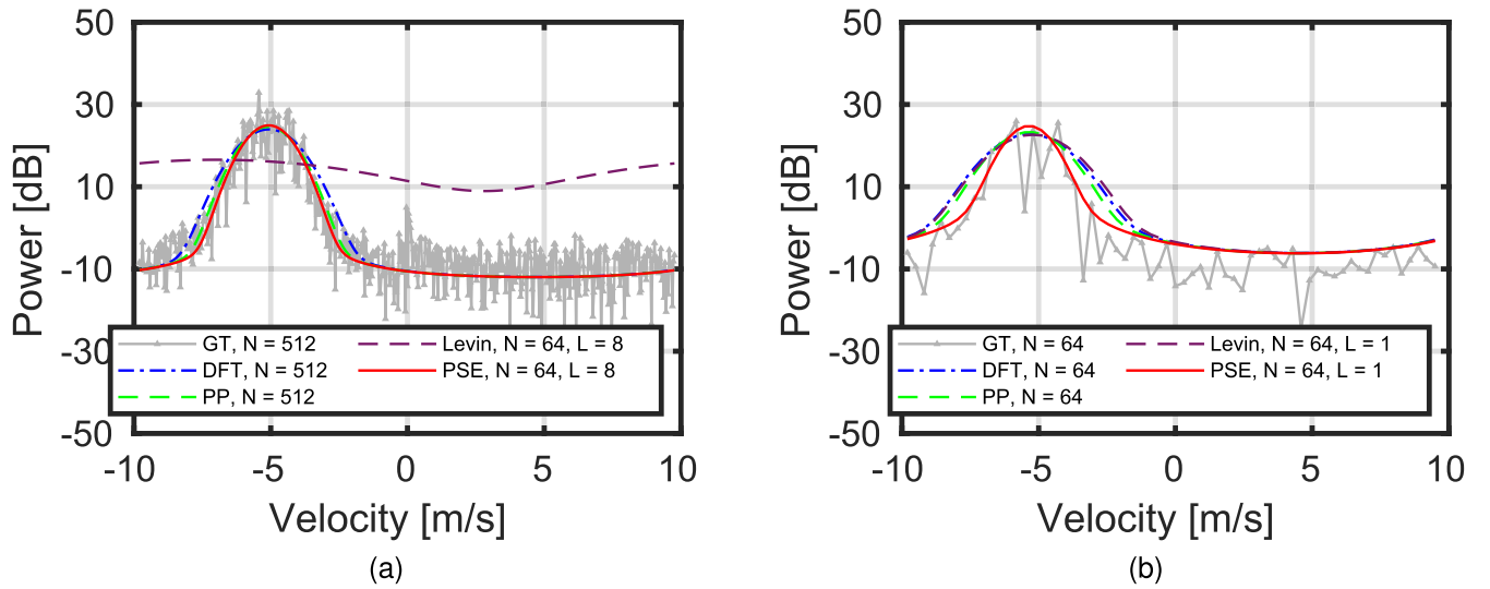
Fig. 8. Doppler spectrum reconstruction at cell (1): (a) 512 total samples and (b) 64 total samples.
