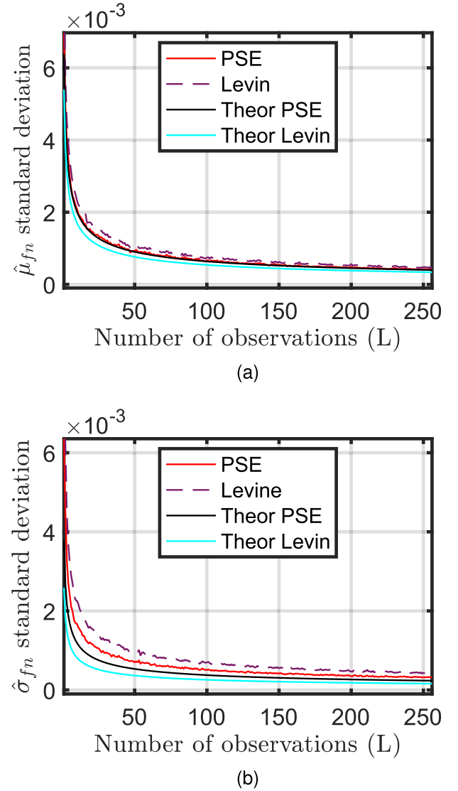
Fig. 4. Estimation and performance of the Doppler moments for N = 64 with respect to L . \mu_{fn} = 0 and \sigma_{fn} = 0.033 (a) Standard deviation in estimating the Mean Doppler Frequency normalized \hat{\mu}_{fn} . (b) Standard deviation in estimating the Doppler Spectrum Width normalized \hat{\sigma}_{fn} .
