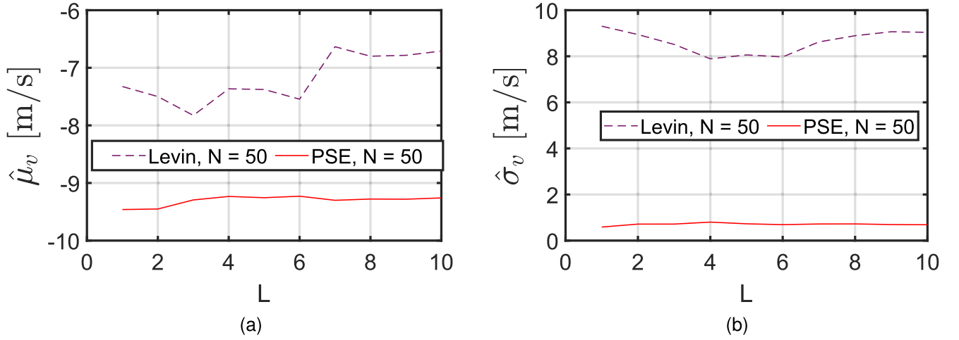
Fig. 14. Doppler moments estimation on real radar data with respect to the number of observations L at resolution cell (2): (a) Mean Doppler velocity \mu_v m/s and (b) Doppler spectrum width \sigma_v m/s.
