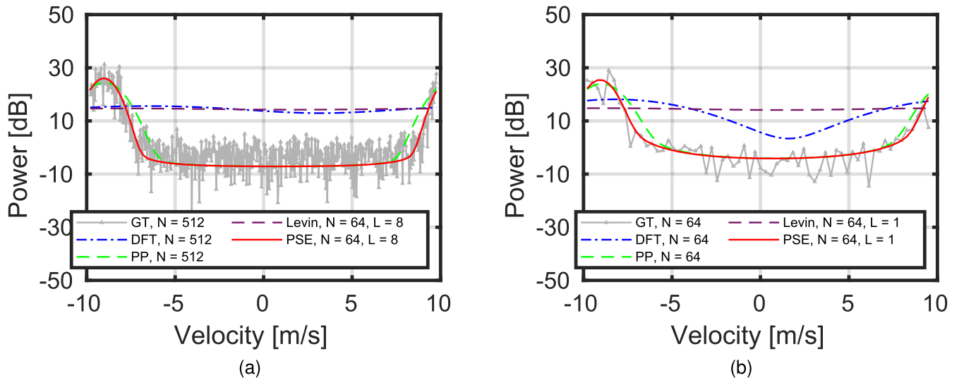
Fig. 9. Doppler spectrum reconstruction at cell (2): (a) 512 total samples and (b) 64 total samples.
