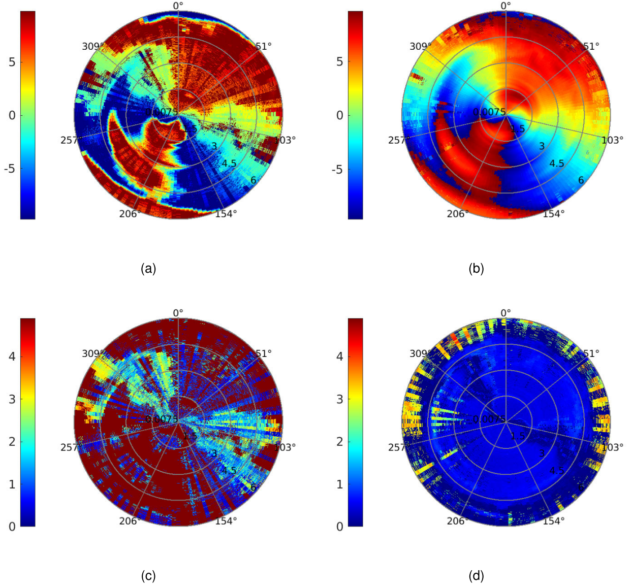
Fig. 16. PPI plots at L = 10 . Incoherent processing of five scans of the radar: (a) mean Doppler velocity \mu_v m/s with Levin's ML approach; (b) mean Doppler velocity \mu_v m/s with PSE; (c) Doppler spectrum width \sigma_v m/s with Levin's ML approach, and (d) Doppler spectrum width \sigma_v m/s with PSE.
