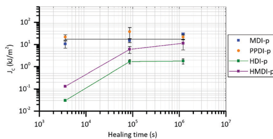
Fig. 6 Long range dynamics effect on fracture resistance recovery. In accordance with time constants obtained from deconvolution, the beneficial effect of long range dynamics is only observed for aliphatic polyurethanes (HDI-p, HDMI-p). Healing temperature is 30^\circ\text{C} .
